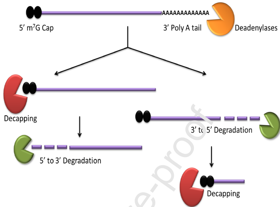
Figure 2: A schematic showing deadenylase dependent pathway of mRNA degradation in eukaryotes. mRNA degradation pathway is initiated by removal of 3' Poly A tail by the deadenylases. The shortening of Poly A tail may lead to 3'-5' exonucleolytic digestion of the mRNA, while decapping is initiated at the 5'-3' end by the exonucleases. The cap structure is cleaved later by the decapping enzymes
