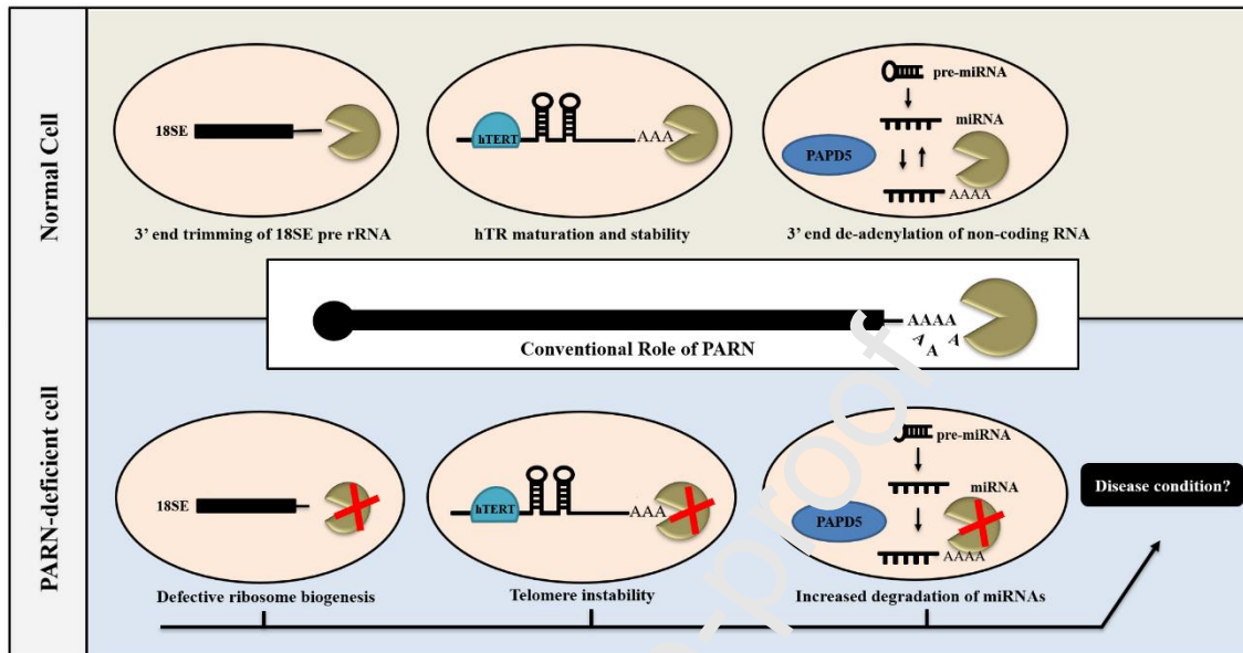
Figure 6: An overview of traditional and emerging functions of PARN. The conventional role of PARN in the removal of adenosine residues from poly-A tails of mRNAs in a 3'-5' direction is shown in the middle of the image. Recent data suggest three emerging roles of PARN, including the processing of the 3'-end of the human 18S rRNA, trimming of oligo-adenylated tails of H/ACA box snRNAs and finally in miRNA processing. These emerging functions of PARN are linked to mRNA translation, telomere maintenance, and ribosome biogenesis, which are deregulated in many disease conditions.
