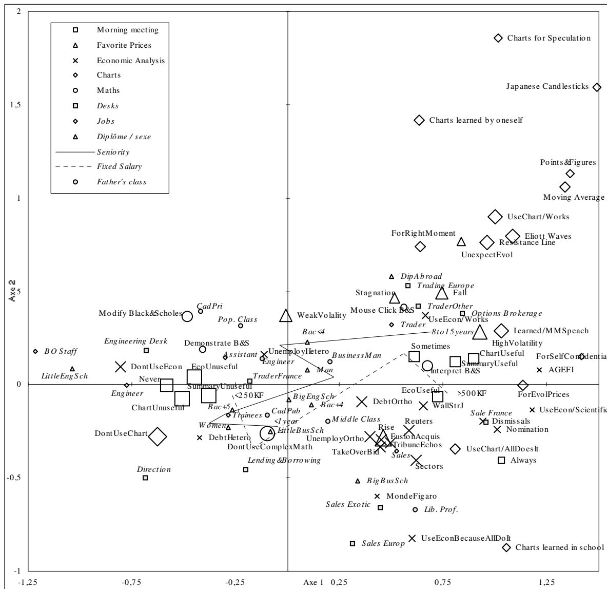
Figure 2. Multiple correspondence analysis of the winning strategies 59 .
