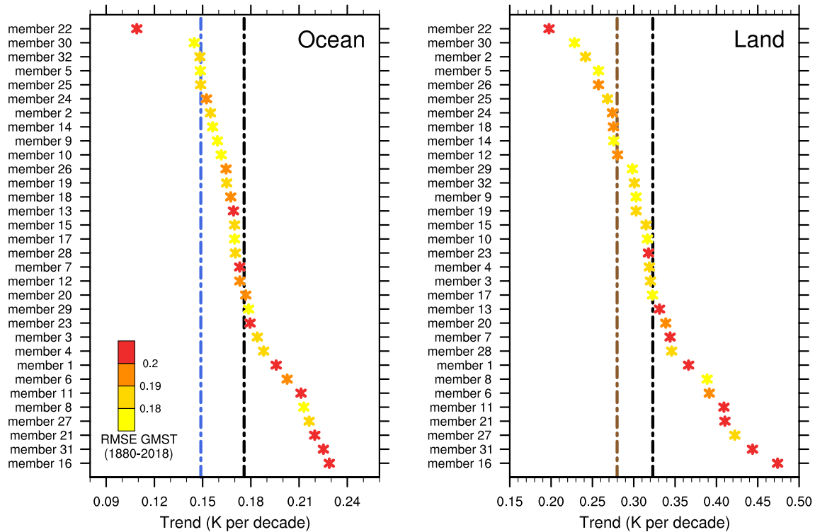
Figure 4. (Left) Trends of average sea surface temperature over the oceans for the 1978–2018 period from the HadSST3 data set of observations (blue dashed line; Kennedy et al., 2011a, 2011b), the ensemble mean of the historical simulations (black dotted line) and the 32 members (stars) ranked from the weakest to strongest trend (from top to bottom). The stars colors are relative to the RMSE of the GSAT (1880–2018). (Right) same as left panel, but for the average land surface temperature using the CruTEM4 observational data set (brown dashed line; Osborn & Jones, 2014).
