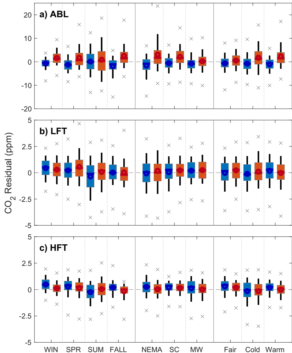
Figure 4. Box and whisker of [\text{CO}_2] residual distributions from CT (blue & left box plots) and WRF (red & right box plots) for seasons, regions, and air masses in (a) atmospheric boundary-layer—ABL; (b) lower free troposphere—LFT; (c) higher free troposphere—HFT. The median and mean are indicated by horizontal lines and circles, respectively. The box indicates 25th and 75th percentiles, whiskers 10th and 90th percentiles, and gray crosses indicate the 2.5th and 97.5th percentiles.
