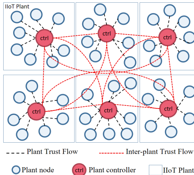
Fig. 1: TM architecture
