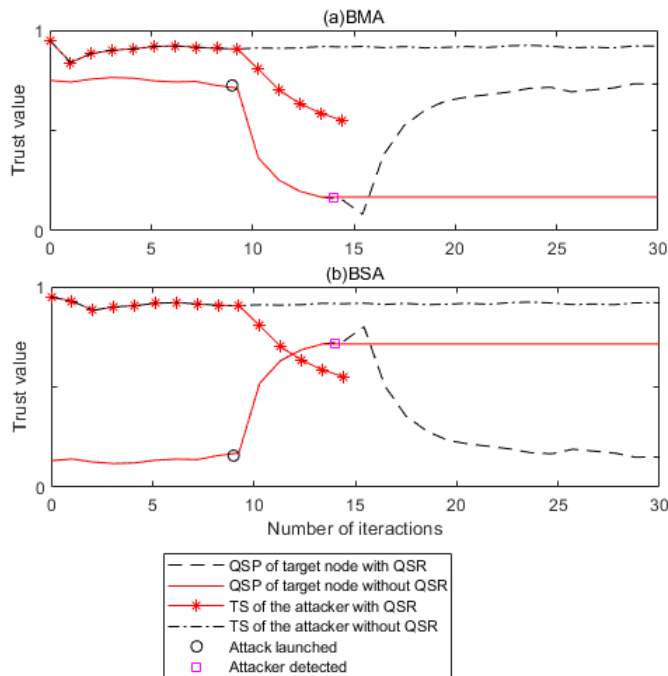
Fig. 14: Changes in trust values of both attacked and attacker nodes with quality of service rater ( QSR ) evaluation and without this evaluation in presence of (a) bad mouthing attack (BMA) and (b) ballot stuffing attack (BSA).
