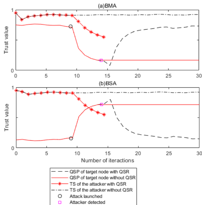
Fig. 15: Changes in trust values of both attacked and attacker nodes with quality of service rater ( QSR ) evaluation and without this evaluation in presence of (a) bad mouthing attack (BMA) and (b) ballot stuffing attack (BSA).
