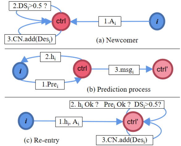
Fig. 6: Checking mechanism and prediction process
