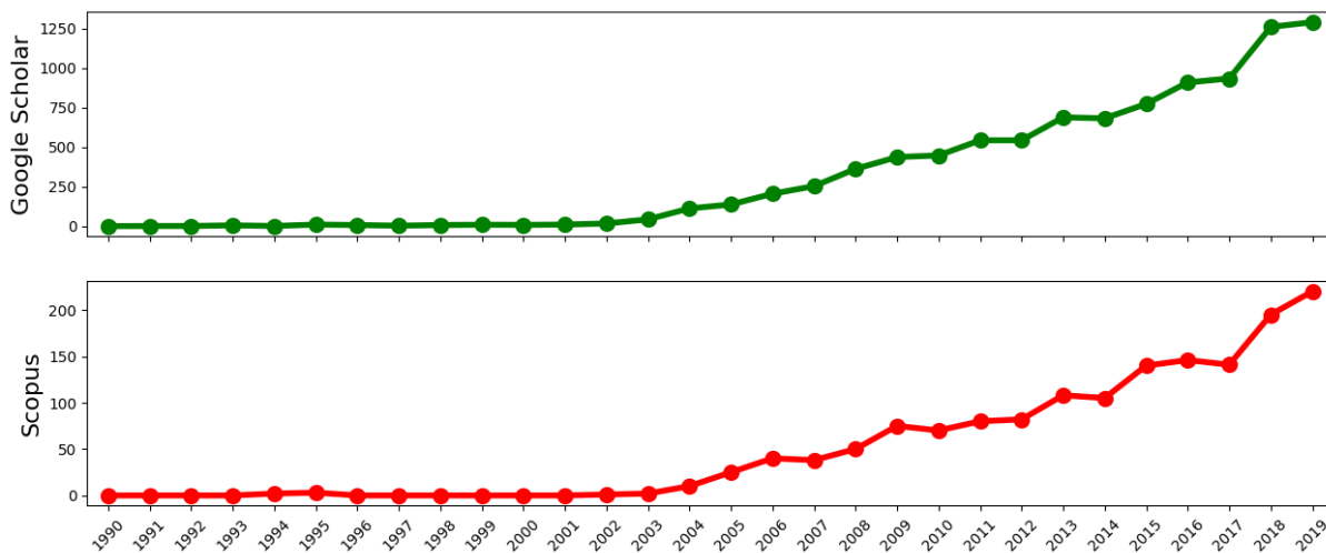
Figure 1: Citation count for the search “swarm robotics” in Google Scholar and in Scopus. Both show the same tendency, with an exponential growth from year 2000 on.
