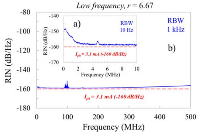
Fig. 5. RIN for 3.1 mA detected photocurrent (sweep points 10001, sweep count 100). The pumping rate, r = I/I_{th} , is 6.67. Red dashed lines are the relative shot-noise level for 3.1 mA detected photocurrent (-160 dB/Hz). a) RIN at very low frequency with RBW = 10 Hz, b) RIN at low frequency with RBW = 1 kHz.
