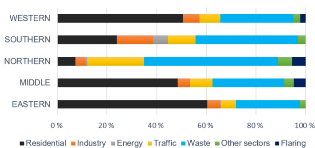
(a) Regional and sectoral contribution to 2015 BC emissions in Africa
