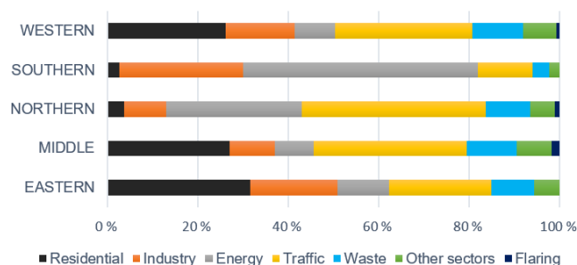
Figure 4. Regional sectoral contribution to 2015 BC (a) and NO x (b) emissions in Africa.
