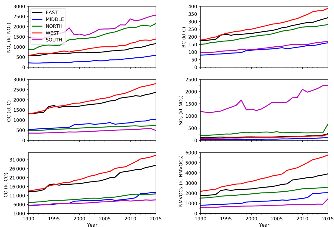
Figure 2. Time series of regional emission estimates of BC, OC, NO x , CO, SO 2 and NMVOCs for fossils fuel, biofuel and waste burning sources.
