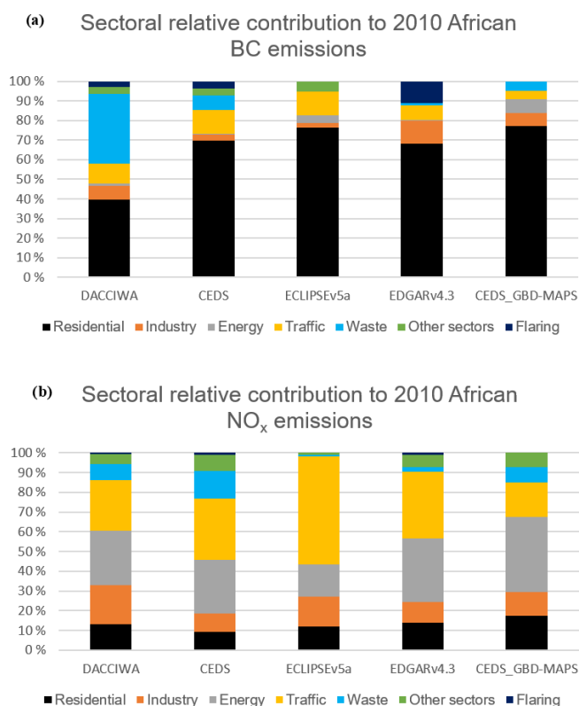
Figure 7. Sectoral relative contribution for BC (a) and NO x (b) emissions in 2010 for CEDS, CEDS_GBD-Maps, ECLIPSEv5a, EDGARv4.3 and DACCIIWA (this work) inventories.
