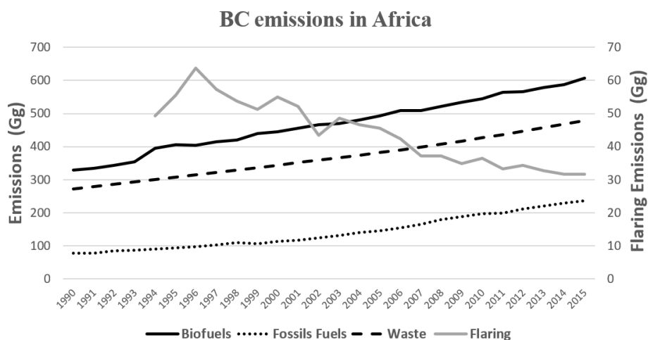
Figure 1. Time series of BC emissions in Africa for fossil fuels, biofuels, open waste burning and flaring.
