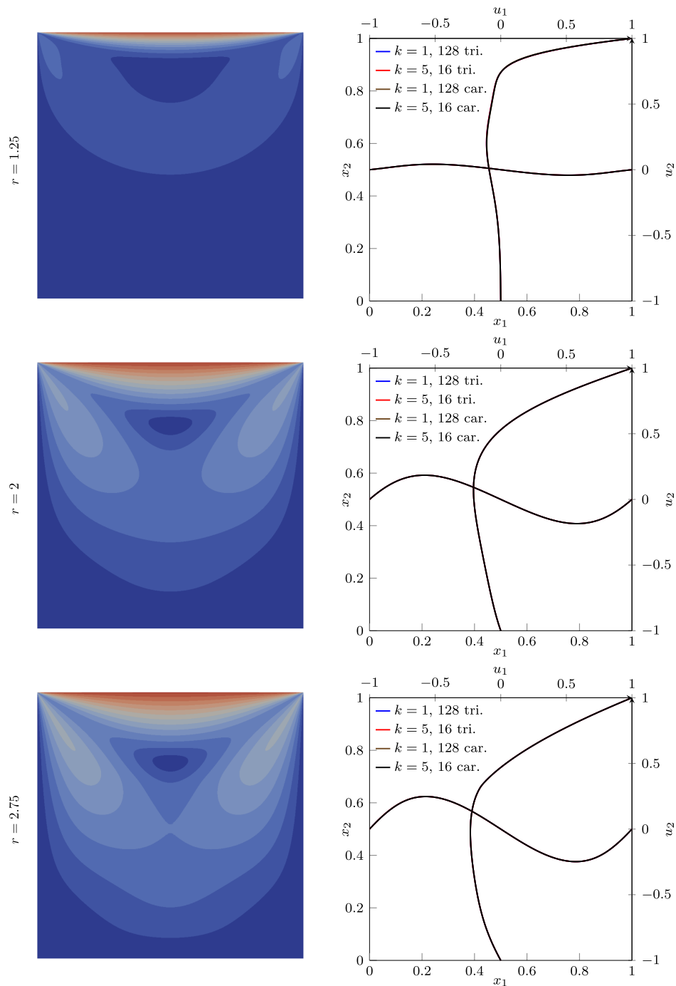
FIGURE 4. Numerical results for the test case of Section 5.2. Left: velocity magnitude contours (15 equispaced values in the range [0, 1] ). Computations on a Cartesian mesh of size 128 \times 128 with k = 5 . Right: horizontal component u_1 of the velocity along the vertical centreline x_1 = \frac{1}{2} and vertical component u_2 of the velocity along the horizontal centreline x_2 = \frac{1}{2} .
