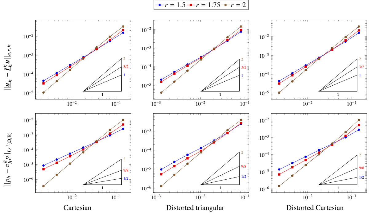
Figure 2: Numerical results for the test case of Section 6. The slopes indicate the expected order of convergence expected from Theorem 20, i.e. \mathcal{O}_{\text{vel}}^1 = 2(r - 1) and \mathcal{O}_{\text{pre}}^1 = 2(r - 1)^2 for r \in \{1.5, 1.75, 2\} .
