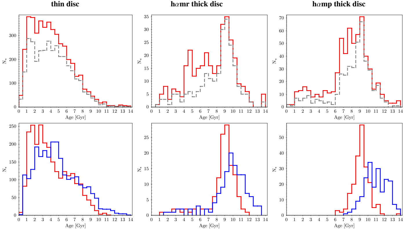
Fig. 7. Age distributions for the thin-, h&mr, and h&mp thick-disc populations, from left to right panels , respectively. Top panels: age distributions from the APOKASC catalogue (red histogram) and with a relative error of less than 25% (grey dotted line). Bottom panels: age distributions from M21 (blue solid line) and from APOKASC (with a relative error less than 25%) for the subsample of stars in common (red solid line).
