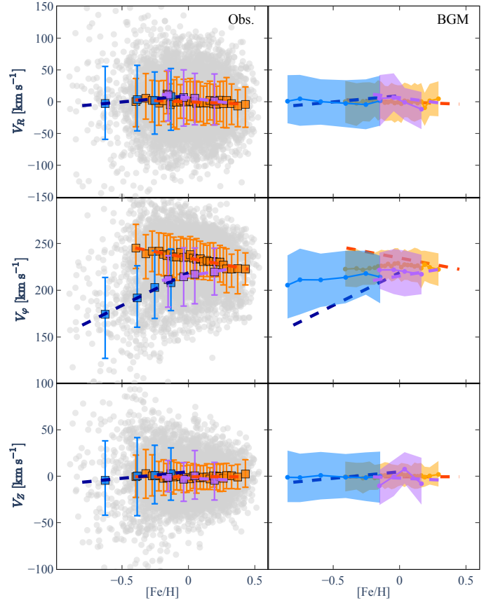
Fig. 11. Velocities in the Galactocentric cylindrical coordinate frame as a function of [Fe/H]. Left panels: all sample stars are shown (grey dots). The mean value per [Fe/H] bin is shown for the thin- (orange), h\alpha mr (purple), and h\alpha mp thick-disc (blue) populations. The mean value has been computed between the 5% and 95% quantiles of the sample to avoid extreme values. The \pm 1\sigma error bars are shown. The dashed lines are the linear fits. Right panels: BGM predictions (orange, purple and blue solid lines) for the APOKASC sample as a function of [Fe/H] compared to the linear fits done using observations (dashed lines). The \pm 1\sigma error bars are shown with the shadow zones.
