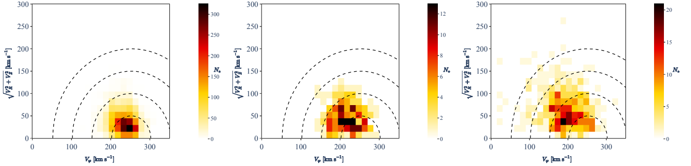
Fig. 9. Toomre diagram for thin-disc (left panel), h α m r thick-disc (middle panel), and h α m p thick-disc (right panel) stars in our sample. The dashed curves indicate constant space motion.
