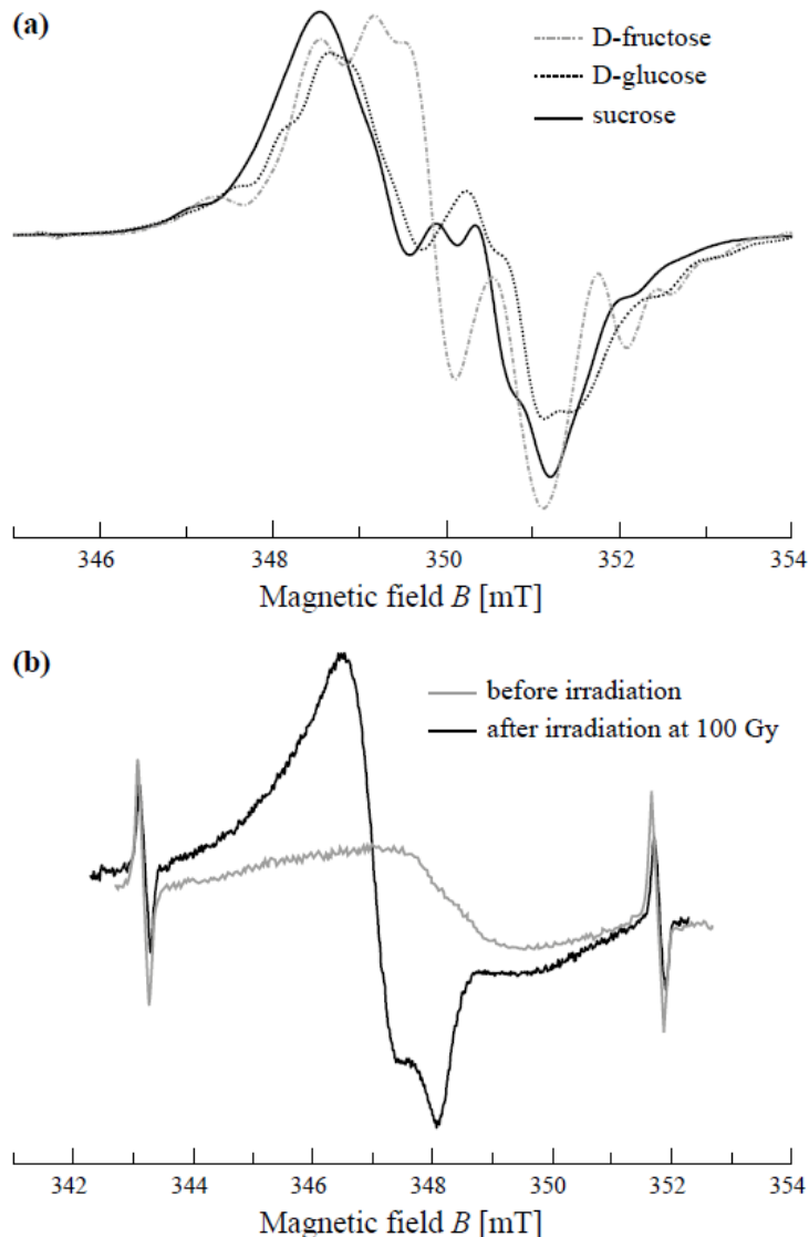
Figure 1.9. X-band EPR spectra for various irradiated samples. a) Samples of sucrose and the two monosaccharides composing it were irradiated at 100 Gy and their spectra were recorded. (b) Soda-lime glass, before and after irradiation at 100 Gy. Spectra were recorded at room temperature at 2 mW.
