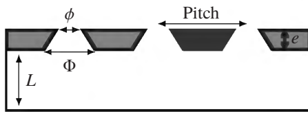
Fig. 2 Geometry of the micro-perforated panel and the plenum.
