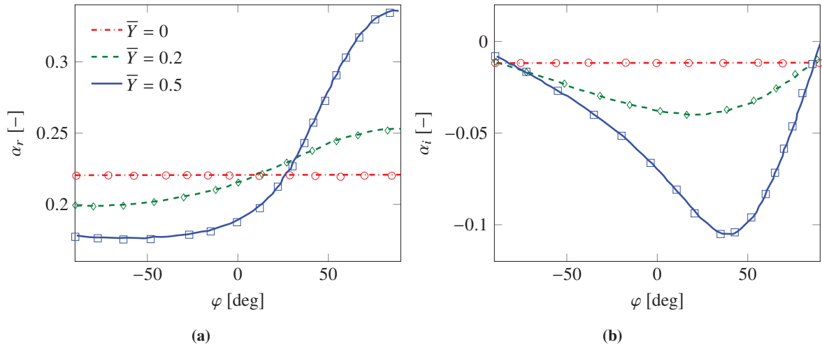
Fig. 13 Variation of (a) \alpha_r and (b) \alpha_i with the phase of admittance for F = 30 \times 10^{-6} and \text{Re}\delta_{\delta_1} = 2240 (corresponding to \omega = 0.0672 ). Lines: present numerical code, Symbols: results from Carpenter and Porter [15] for \bar{Y} = 0 ( \circ ), \bar{Y} = 0.2 ( \diamond ) and \bar{Y} = 0.5 ( \square ).
