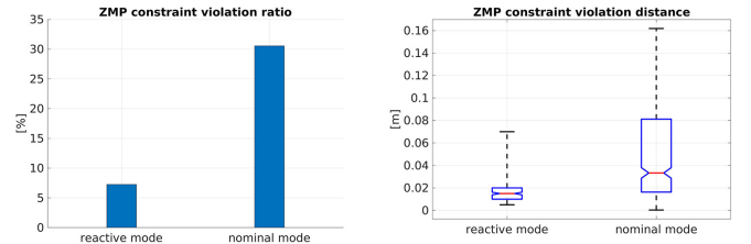
Fig. 8. A straightforward illustration of walking stability in test-1. Left: The proportion of the sampled data where the ZMP constraint is not satisfied. Right: The shortest distance between the ZMP and the corresponding SP for the unstable sample instants.
