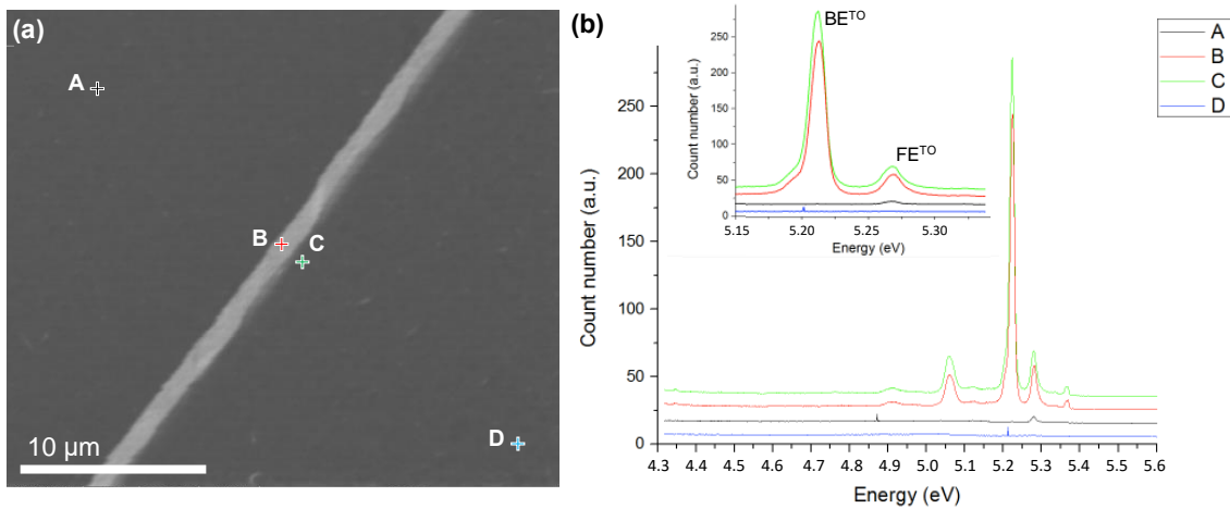
Figure 2. (a) SEM micrograph of the region where spectra are recorded with the specific positions marked. (b) CL spectra of the four positions shown in the SEM micrograph.
