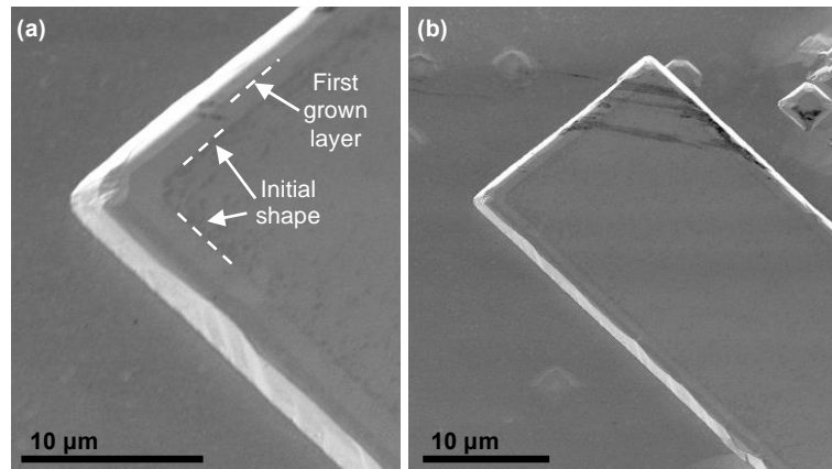
Figure 1. SEM micrographs of the grown sample tilted 35^\circ . Two contrast are observed, one attributed to the initial shape and another, less obvious, due to the change in the surface orientation. Both are visible at the edges of the structure and marked in (a).
