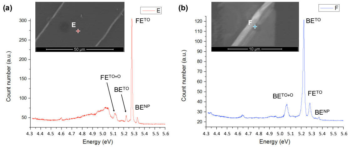
Figure 3. CL spectrum at the positions marked with a cross in the SEM micrographs shown as inset. (a) Spectrum recorded in an area of the sample growth vertically along the (100) orientation. (b) Spectrum recorded in an area of the sample growth laterally. Main peaks are identified.
