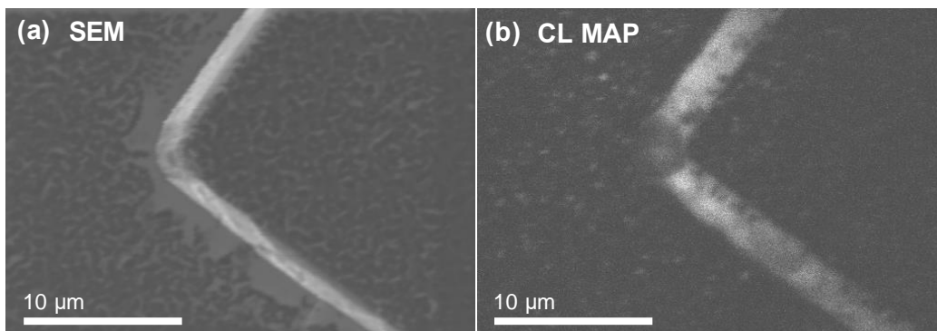
Figure 4. (a) SE-SEM micrograph of one of the corner of a mesa rectangle. (b) Monochromatic CL map of the \text{BE}^{\text{TO}} peak (5.210 eV) corresponding to the same region of the sample.
