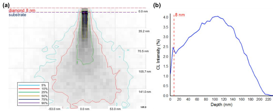
Figure 5. (a) Monte Carlo simulation of the energy by position in a 5 keV accelerating voltage beam impinging a bi-layered diamond sample. (b) CL intensity per depth of the same simulation.
