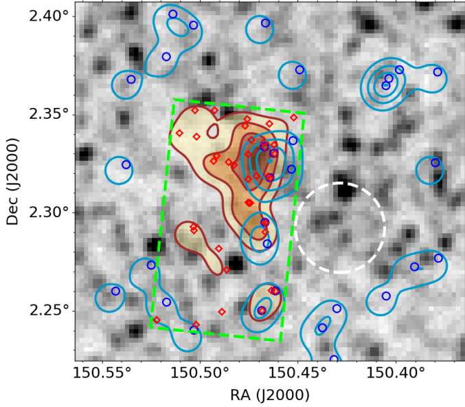
Fig. 3. Spatial distribution of spectroscopic sources (blue circles), and HAEs (red diamonds) overlaid on the SPIRE 350 \mu\text{m} image of the G237 field. The yellow-brown filled contours show the HAE projected density, and the turquoise contours show the projected density of the spectroscopic sources. The density contour levels are shown at 25, 50, 75, and 100% of the maximum value. The dashed green rectangle represents the MOIRCS field of view where the HAE were selected (Koyama et al. 2021). The spectroscopic and HAE density peaks are 38'' apart. The white circle represents a masked region in the L16 catalog due to the presence of a bright star.
