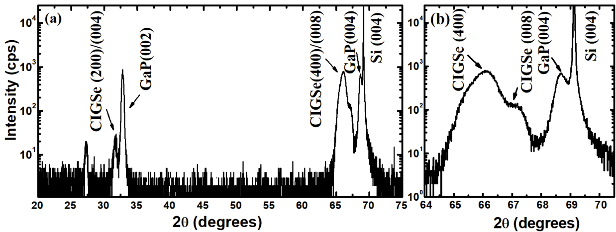
Figure 4: \omega/2\theta longitudinal scan on the CIGSe/GaP/Si sample. (a) wide \omega/2\theta scan displaying intense (00l) and (h00) reflections with even h and l, compatible with the CIGSe chalcopyrite structure (b) Focus around the GaP(004) peak showing evidence of the tetragonal splitting of the CIGSe(400) and CIGSe(008) reflections
