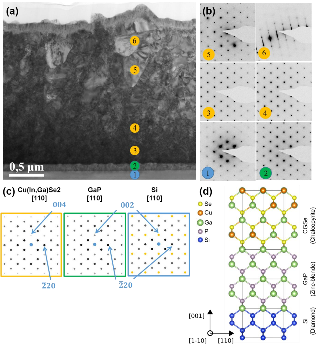
Figure 8: (a) Cross section TEM bright field micrograph. (b) Selected area electron diffraction patterns acquired in Si substrate (1), GaP layer (2) and CIGSe layer (3 to 6). (c) Simulated electron diffraction patterns of Si, GaP and CIGSe crystalline structures along [110]. (d) Corresponding schematic of the crystalline structures stacking considering the CIGSe a -matched crystallographic variant. The figure represents the pure-Ga CGSe chalcopyrite structure for simplicity's sake
