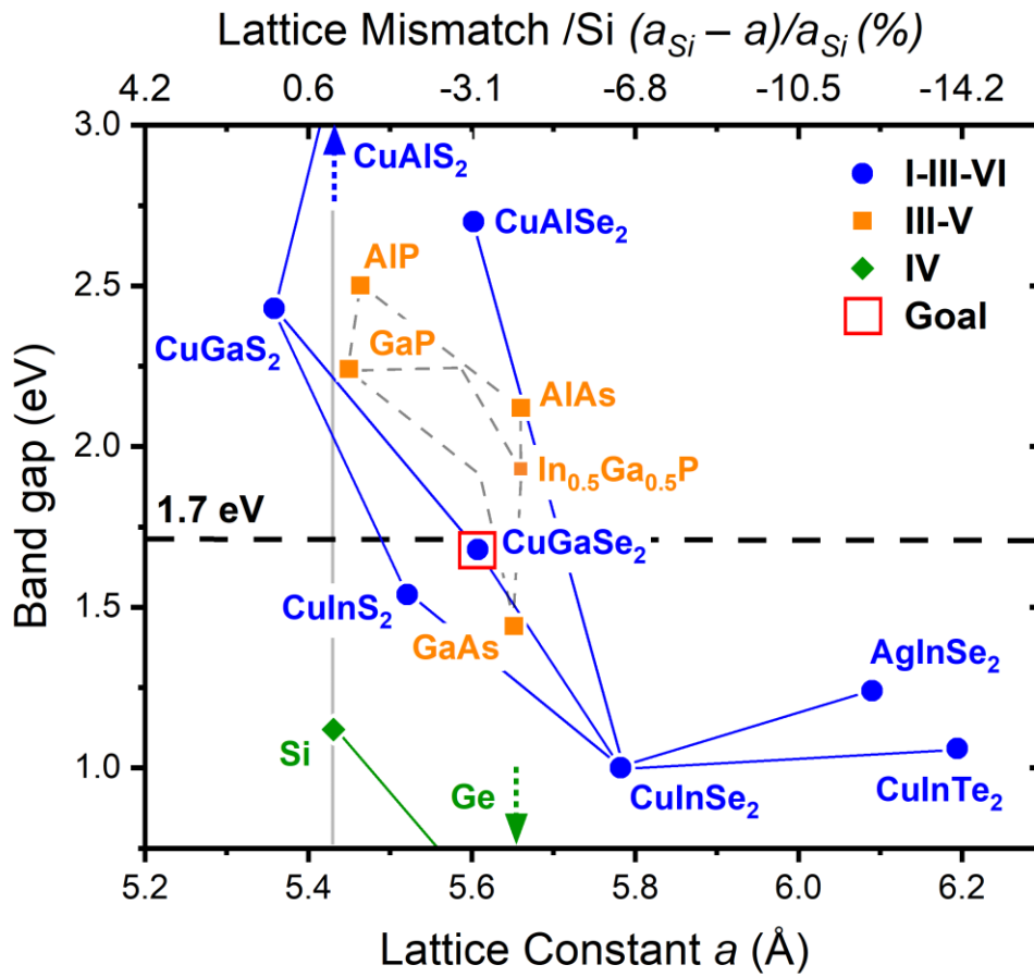
Figure 2: Band gap vs lattice mismatch for chalcopyrites, silicon and III-V [14]. Gallium phosphide GaP is quasi lattice matched with Si. Additionally, in the Cu(In,Ga)(S,Se) 2 family, pure-Ga CIGSe selenides have near ideal band gap for top cell applications. Lattice mismatch relative to a_{Si} the lattice constant of Si is represented on the top x-axis scale.
