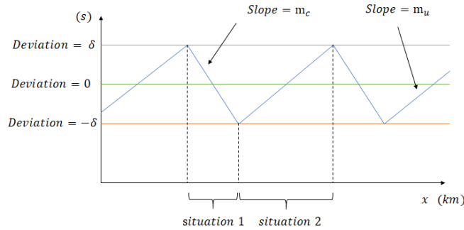
Fig. 1. Basic driving process of the bus with CSP
