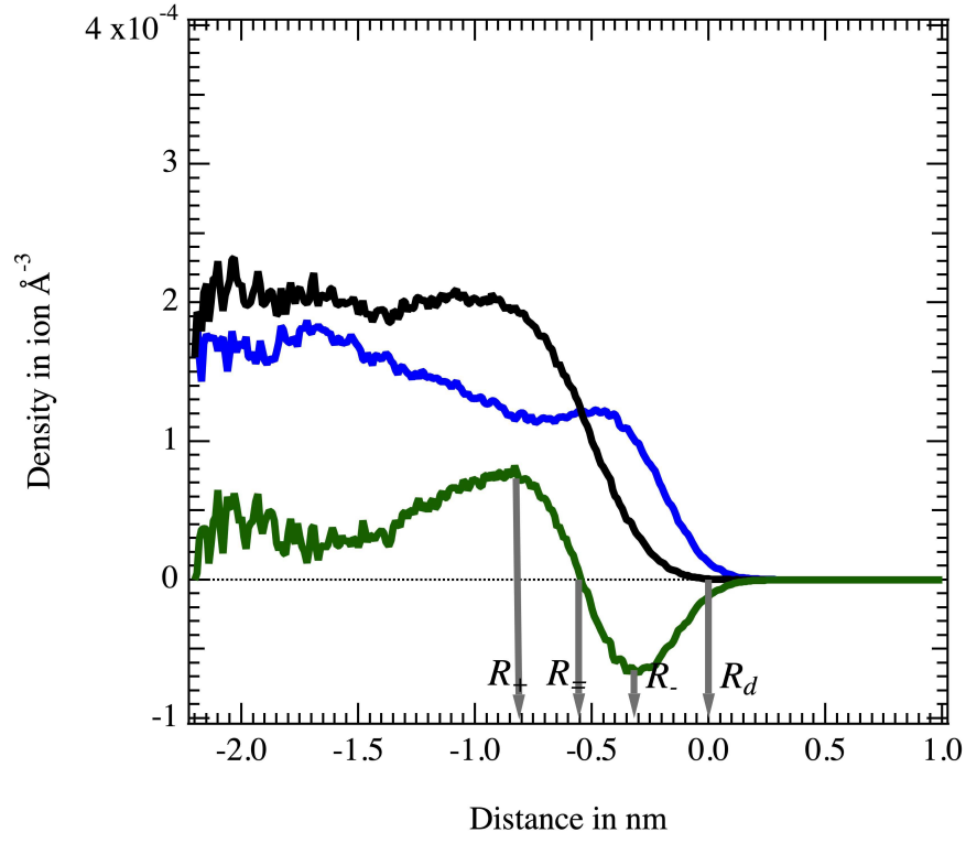
Figure S6: Ion densities as a function of the ion distance from the equi molar radius R_d for the 2k 0.2m droplet. \text{Na}^+ and \text{Cl}^- densities are plotted in black and blue lines, respectively. Green line: difference \Delta\rho^i(r) in the \text{Na}^+ and \text{Cl}^- densities. The vertical grey arrows are located at the minimum, zero and maximum values of the \Delta\rho^i(r) function and at the mean droplet radius R_d .
