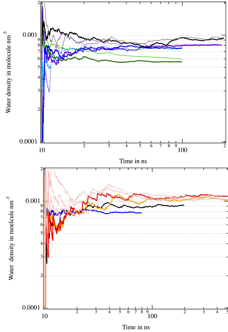
Figure S13: Up : temporal evolutions of the water vapor density for the 0.2m (thin lines) and 0.6m (bold lines) 5k (black), 10k (violet), 20k (blue) and 100k (green) salty droplets. Down : temporal evolutions of the water vapor density for 1k (red bold and thin lines, each line corresponds to an independent 500 ns simulation), 5k (orange), 10k (black) and 20k (blue) pure aqueous droplets.
