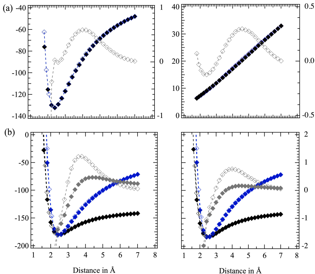
Figure S3: (a) [\text{Na}^+, \text{Cl}^-] ion pair interaction energy (in kcal mol -1 , plot on the left) and total dipole moment (in Debye, plot on the right) in gas phase as a function of the inter ionic distance from ab initio MP2/CBS computations (full black symbols) and from our force field (empty blue symbols). Dashed grey lines and symbols: differences between force field and ab initio data (right axes). (b) Interaction energies (in kcal mol -1 ) of the ionic trimers [(\text{Na}^+)_2, \text{Cl}^-] (left) and [\text{Na}^+, (\text{Cl}^-)_2] (right). In these trimers, the single ion is set in between the two ions of opposite charge. Full and empty symbols: quantum and force-field data, respectively. Blue symbols (left axis): trimer interaction energies corresponding to symmetric dissociation of the two charge-like ions. Black symbols (left axis): trimer interaction energies corresponding to the dissociation energy of one of the two charge-like ions. Grey lines and symbols (right axes): force field/quantum differences in the trimer energies.
