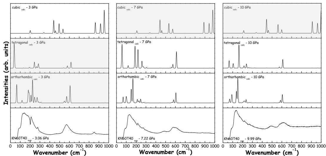
Figure 8. Calculated and experimental Raman spectra for \text{KNb}_{0.6}\text{Ta}_{0.4}\text{O}_3 at 3 GPa, 7 GPa and 10 GPa (from left to right). For each pressure, theoretical spectra were calculated with orthorhombic, tetragonal and cubic symmetries. Grey area corresponds to the best agreement between DFT calculations and theoretical datas
