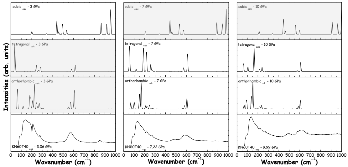
Figure 8. Calculated and experimental Raman spectra for KNb 0.6 Ta 0.4 O 3 at 3GPa, 7GPa and 10GPa (from left to right). For each pressure, theoretical spectra were calculated with orthorhombic, tetragonal and cubic symmetries. Grey area corresponds to the best agreement between DFT calculations and theoretical datas
