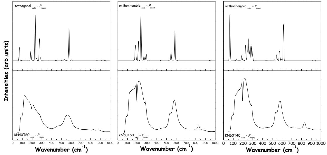
Figure 5. Calculated (up) and experimental (down) Raman spectra for \text{KNb}_{1-x}\text{Ta}_x\text{O}_3 ( x=0.6, 0.5 and 0.4 from left to right) at room pressure.
