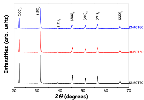
Figure 1. X-ray diffraction patterns of \text{KNb}_{1-x}\text{Ta}_x\text{O}_3 polycrystalline samples in the perovskite phase.
