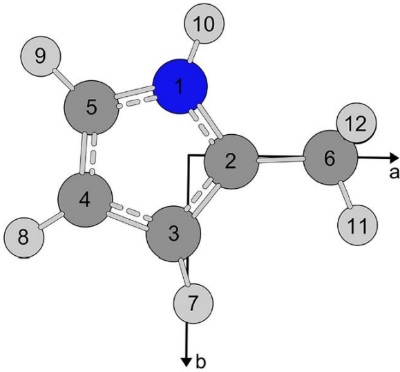
Figure 1. The molecular geometry of 2MP optimised at the MP2/cc-pVDZ level of theory. The atom numbering and the a and b inertial principal axes of inertia are given. The hydrogen atom H 13 is located behind H 12 .
