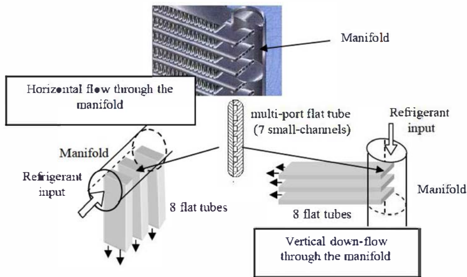
FIG. 1 – Distributor for small-channel heat exchangers used in industrial applications.
