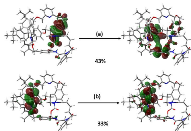
Figure 9. Natural Transition Orbital pairs for the 240 nm band for conformer C463. Ground state MO density is on the left and the corresponding excited state density is on the right. (a). The contribution from the top pair (a) is 43% and that from the bottom pair (b) is 33%.
