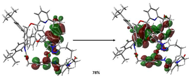
Figure 7. Natural Transition Orbitals for the 240 nm ECD band of conformer C269. The electron density in ground state MO is on the left, and that in the corresponding excited state MO is on the right. The contribution from this pair is ~78%.
