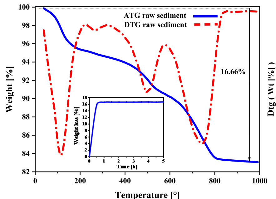
Figure 3. Sediment weight loss variation with time and temperature.
