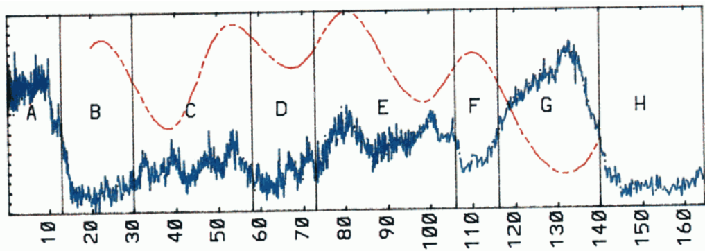
Plate 1. ESA analysis of the temperature time series at Vostok. The left axis represents the middle of the moving windows and the colors give the degree of confidence. The corresponding temperature time series is plotted on the left, in blue. The global high-frequency variability of the time series is plotted on the same scale, for comparison purposes, in red.
