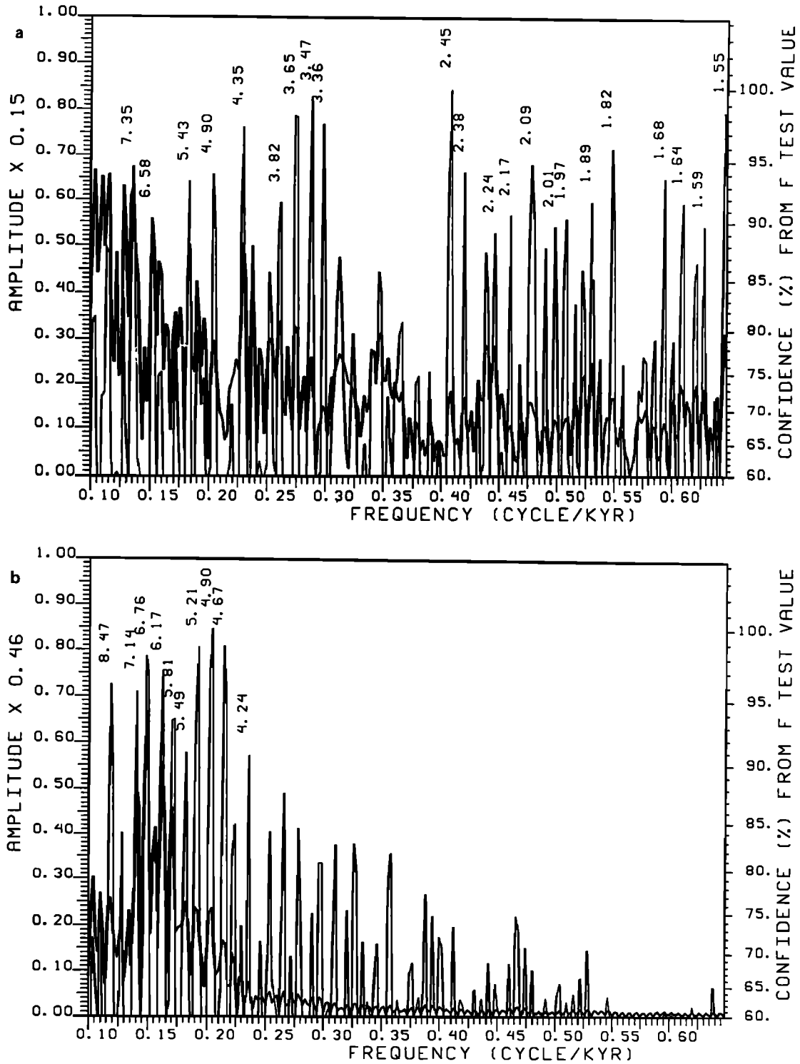
Fig. 3. (a) MTM analysis of the temperature time series at Vostok for higher frequencies. Thick and thin curves as in Figure 2. (b) MTM analysis of the temperature time series from the GLT model. The frequency band is 0.1–0.65 cycles/kyr in both panels.
