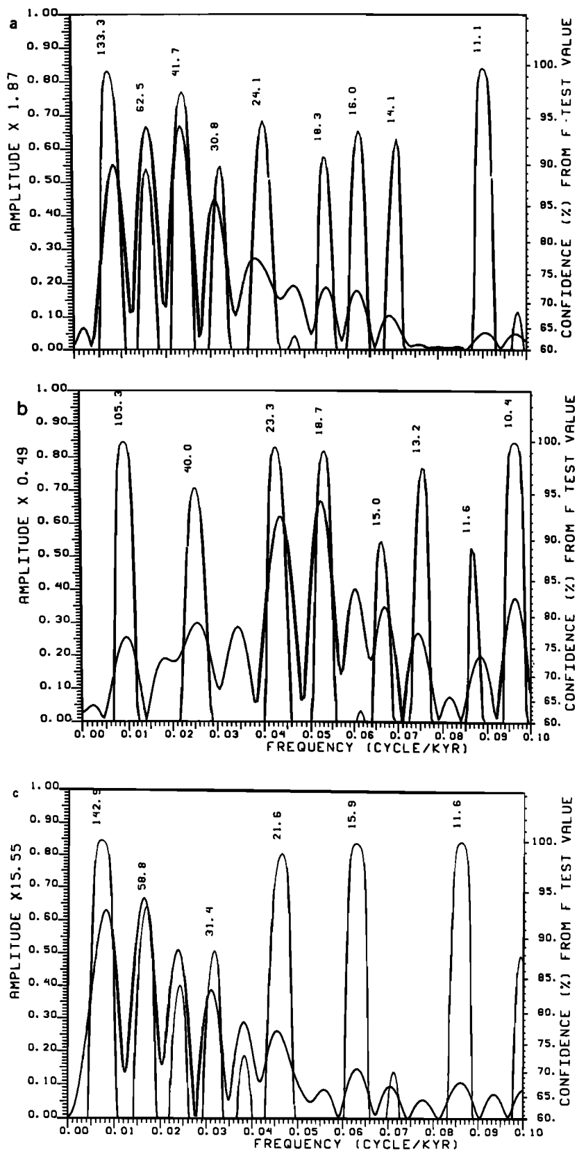
Fig. 2. (a) MTM analysis of the entire temperature time series at Vostok. The thick curve represents the amplitude (left axis) and the thin curve represents the confidence value in percent (right axis). (b) MTM analysis of the temperature from the Ghil-Le Treut (GLT) model [Ghil and Le Treut, 1981; Le Treut and Ghil, 1983]. The time series analyzed is 164 kyr long and sampling is at 0.5 kyr. (c) MTM analysis of the CO 2 time series at Vostok. The frequency band is 0 to 0.1 cycles/kyr in all three panels.
