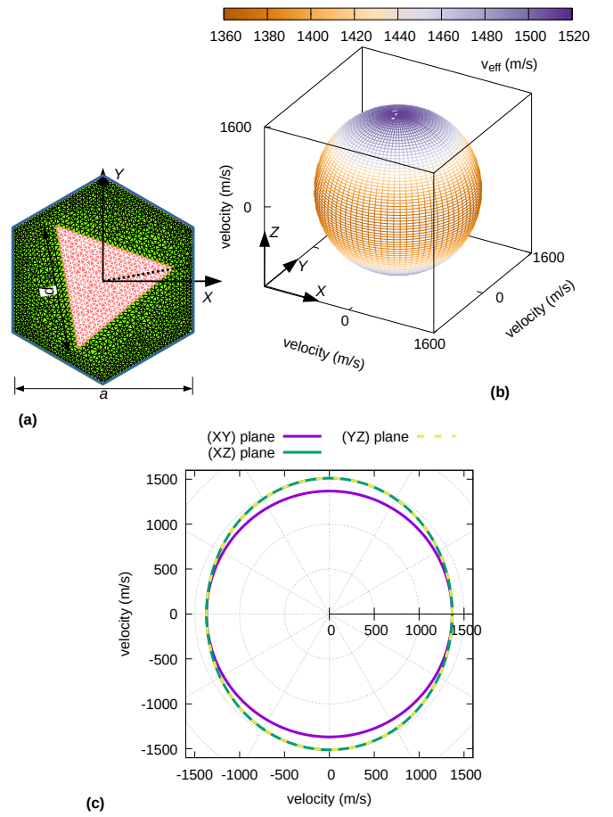
Figure 3. (a) A 2D hexagonal-lattice sonic crystal composed of triangular steel rods in water. The triangular rods are rotated by 10^\circ with respect to the X axis. The ratio of the length of the equilateral triangle to the lattice constant is d/a = 0.7 . The crystal has a C_3 symmetry and is transverse isotropic. (b) Effective velocity surface. (c) Cross-sections through the symmetry planes of the crystal.
