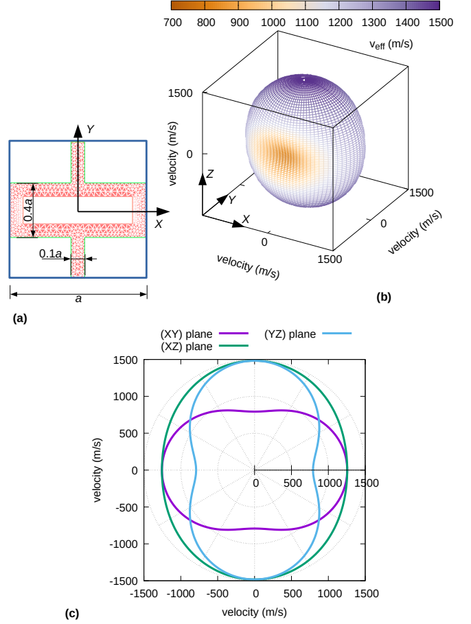
Figure 5. (a) A 2D sonic crystal composed of a periodic array of waveguides containing water. The crystal is orthotropic with three independent tensor elements. (b) Effective velocity surface. (c) Cross-sections through the symmetry planes of the crystal.
