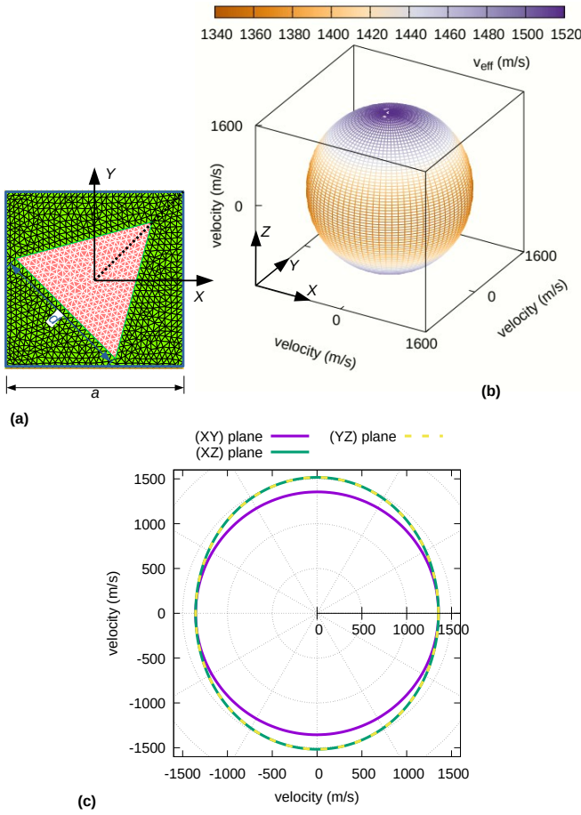
Figure 2. A 2D square-lattice sonic crystal composed of triangular steel rods in water. (a) The triangular rods are rotated by 45^\circ with respect to the X axis. The ratio of the length of the equilateral triangle to the lattice constant is d/a = 0.8 . The crystal is orthotropic. (b) Effective velocity surface. (c) Cross-sections through the symmetry planes of the crystal.
