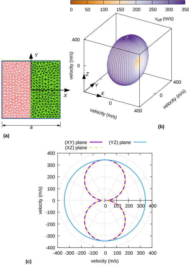
Figure 4. (a) A laminar 1D sonic crystal composed of alternated layers of water and air with equal thickness. The structure is invariant along axes Y and Z . The crystal is orthotropic with two independent tensor elements. (b) Effective velocity surface. (c) Cross-sections through the symmetry planes of the crystal.
