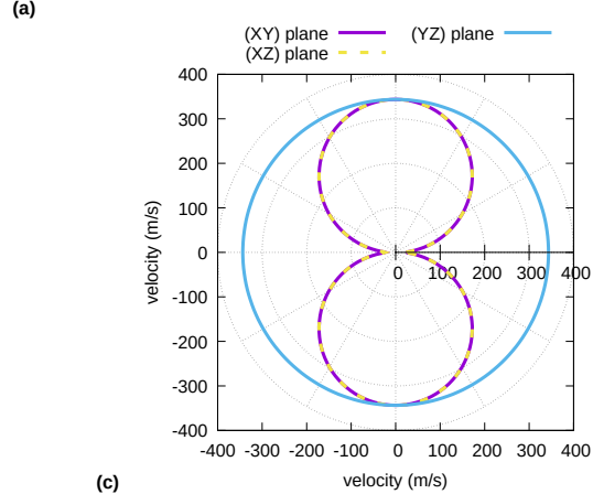
Figure 4. (a) A laminar 1D sonic crystal composed of alternated layers of water and air with equal thickness. The structure is invariant along axes Y and Z . The crystal is orthotropic with two independent tensor elements. (b) Effective velocity surface. (c) Cross-sections through the symmetry planes of the crystal.
