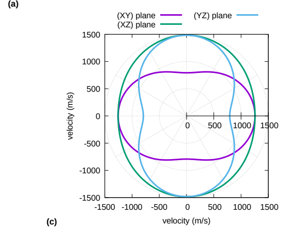
Figure 5. (a) A 2D sonic crystal composed of a periodic array of waveguides containing water. The crystal is orthotropic with three independent tensor elements. (b) Effective velocity surface. (c) Cross-sections through the symmetry planes of the crystal.
