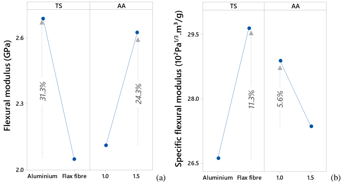
Figure 6. Main effect plots for flexural modulus (a) and its specific property (b).
