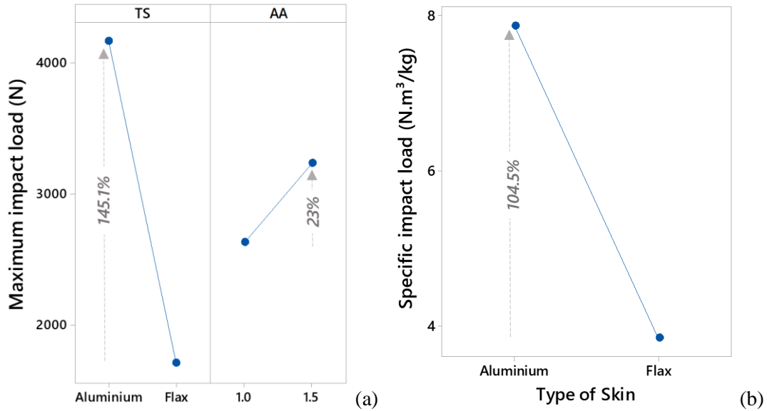
Figure 8. Main effect plots for absolute (a) and specific impact load (b).
