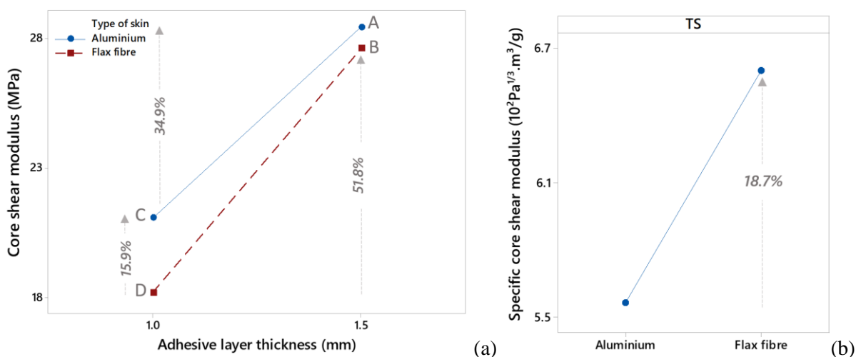
28 Figure 5. Interaction and main effect plots for core shear modulus (a) and its specific modulus (b).
