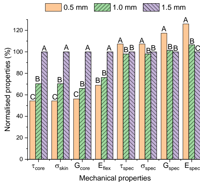
16 17 Figure 7. Normalised mechanical properties for the independent test with flax fibres.
