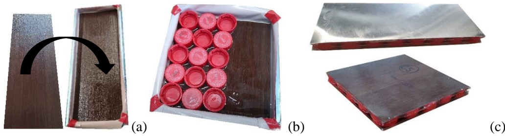
Figure 1. Manufacturing process for sandwich panels: finished skins in the mould (a), bonding of caps core (b) and finished samples of both skins for flexural and impact tests (c).
