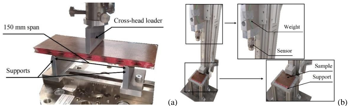
Figure 2. Experimental setup: flexural (a) and drop-tower impact test (b).
