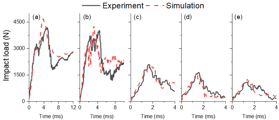
Figure 13. Force vs time results of dynamic experiment and FE models for the conditions 1 to 5 (a - e, respectively).
