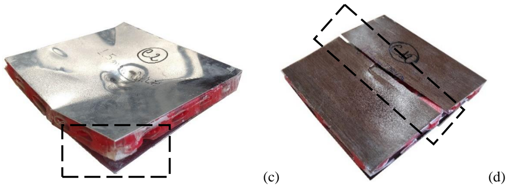
Figure 11. Failure mode of aluminium (a, c) and flax-based panels (b, d) under flexural and impact, respectively.
