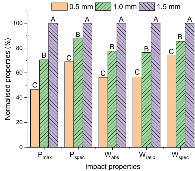
Figure 10. Normalised impact properties for the independent test with flax fibres.
