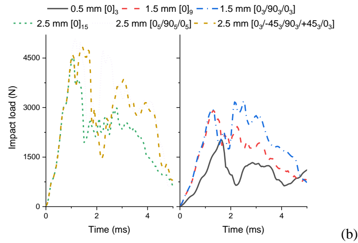
Figure 15. Quasi-static (a) and dynamic (b) response of model with thicker multidirectional laminates.
