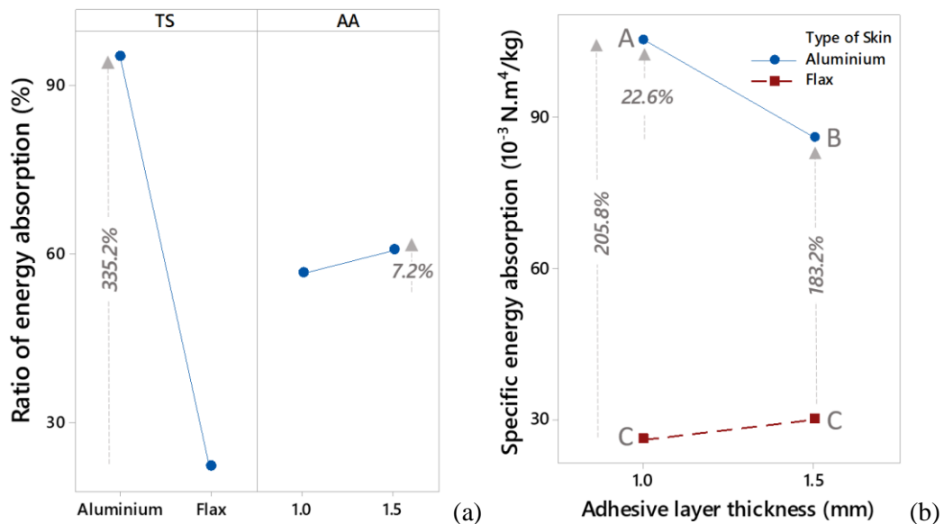
Figure 9. Interaction plots for energy absorption ratio (a) and specific energy absorption (b).
