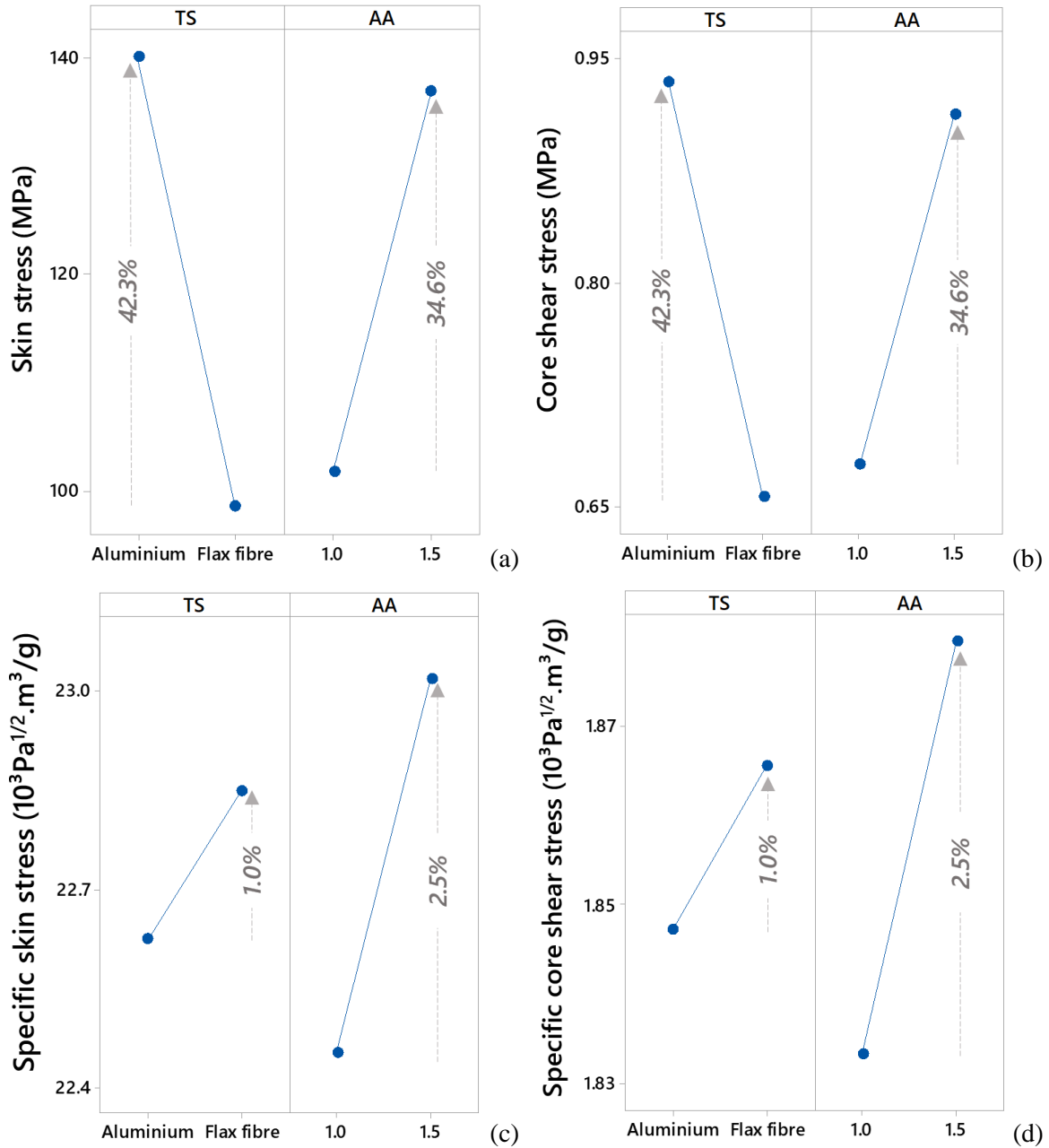
Figure 4. Main effect plots for skin stress and core shear stress (a, b) and their specific properties (c, d).
