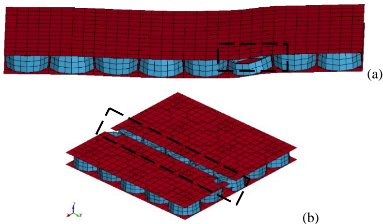
Figure 14. Failure of samples obtained via FEA for conditions C3 for quasi-static (a) and dynamic test (b).
