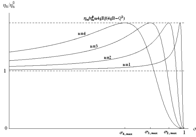
Fig. 2 – Deflections \eta_n caused by internal gravity waves under ice cover as a function of normalized frequency \sigma = \omega / N . Each profile is normalized by amplitude \eta_n^0 at \omega = 0 .
