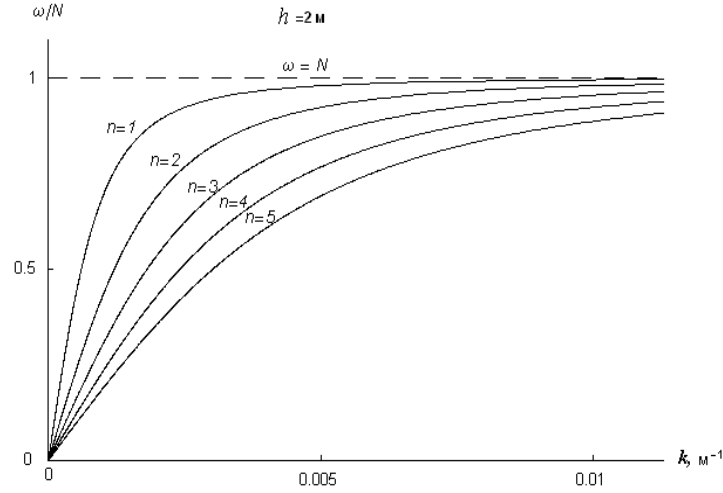
Fig. 1 – Dispersion curves \omega_n(k) for internal gravity waves under an ice cover of constant thickness h = 2 m. The plots were made for an ocean with depth H = 3000 m and Brunt–Väisälä frequency N = 0.001 s -1 .
