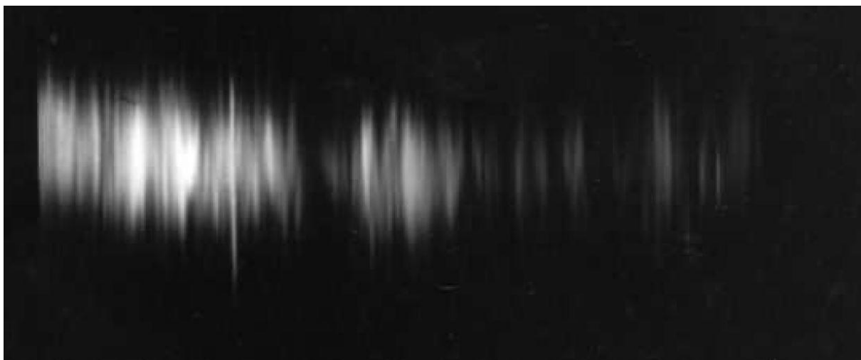
Figure 13: Spectra of spicules (chromospheric plasma jets) at the limb in H \alpha obtained with a curved slit by Z. Mouradian, revealing the Doppler effect. The wavelength is in the y-direction (courtesy: OP).
