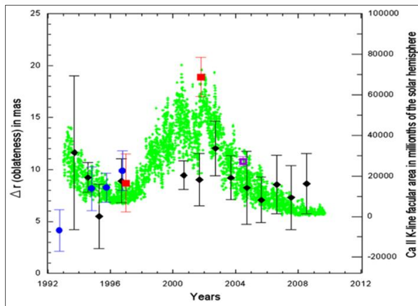
Figure 27: Solar flattening (difference \Delta r between the equatorial and polar radius) as deduced from Pic du Midi observations (diamonds), Solar Disk Sextant (SDS) balloon flights (circles), SOHO-MIDI (squares) and RHESI space measurements (hollowed out square), plotted together with the faculae area index (green) produced by San Fernando Observatory (USA), as a function of time (after Damiani et al., 2011: 247).
