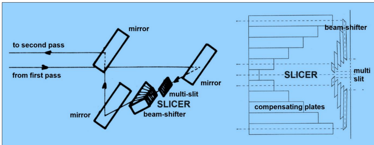
Figure 14: The MSDP device. Left: the slicer in the spectrum is composed of two parts, the beam-splitter (multi-slit) and the beam-shifter which realigns the beams for the subtractive pass on the grating. Right: details of the slicer (the beam-shifter is made of prisms and compensating plates) (after Mein, 1980: 289 ).
