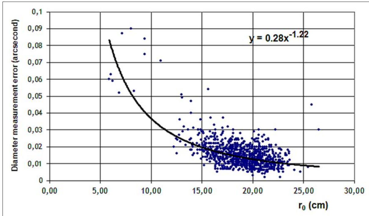
Figure 26: Error in diameter measurements as a function of the Fried parameter r_0 (a parameter characterizing the turbulence, values above 15 cm correspond to good seeing conditions). Data recorded on 6 September 2001, with exceptional weather conditions. Note that the theoretical diffraction limit of the refractor is 0.256'' . The exponent of the fitting is 1.22, close to the theoretical value (1.20). Two points have been obtained for high values of r_0 (i.e., 25.7 and 26.4 cm), which are out of the fitting and probably erroneous (after Rozelot et al., 2003: 45).
