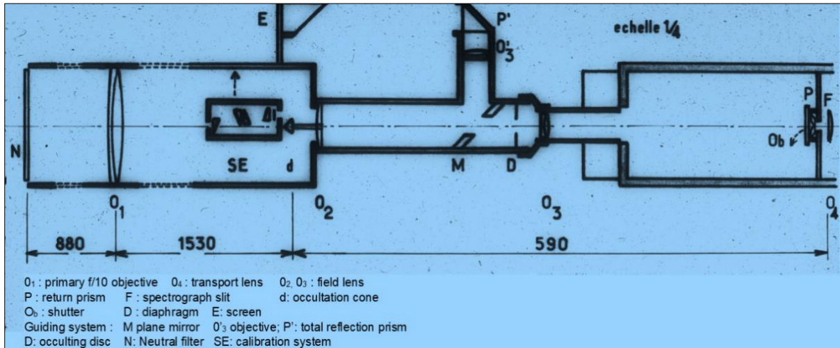
Figure 19: The 0.15 m coronagraph at F/10 designed by J. Rösch in 1964 (the spectrograph is not drawn, the entrance slit F is indicated at right) (courtesy: OCA).
