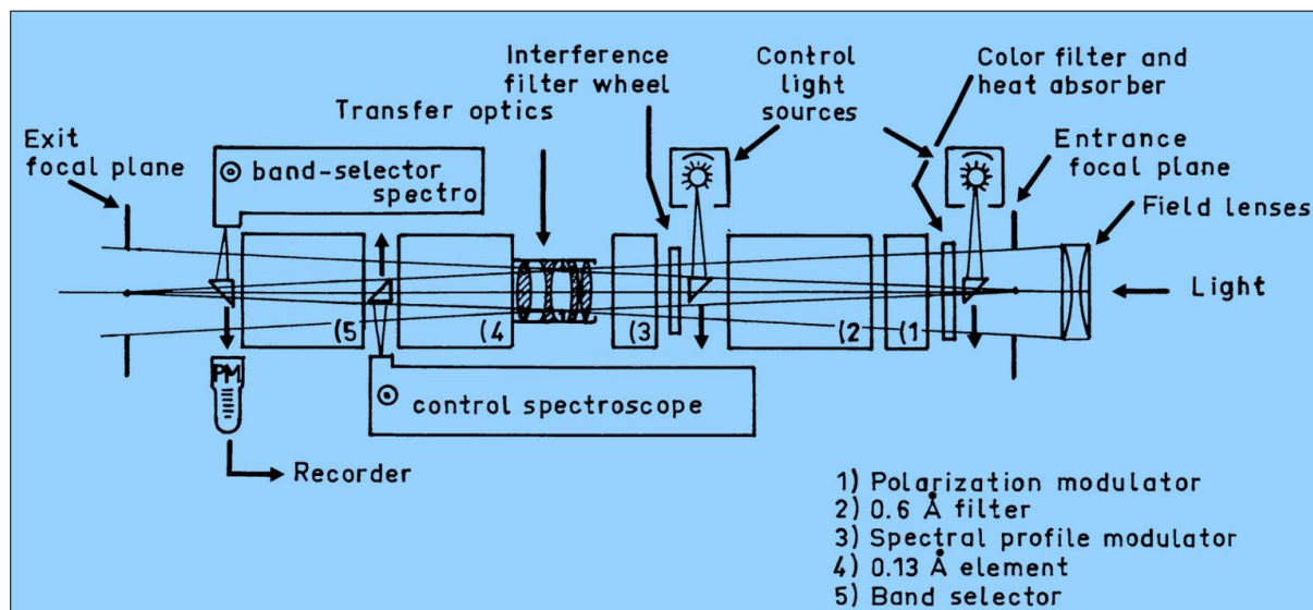
Figure 8: The 'Filtre Polarisant Solaire Selectif' (FPSS) developed at Meudon and installed on the Turret-Dome in 1992 was composed of two Lyot filters and a polarization modulator (after Dollfus et al., 1985: 242).
