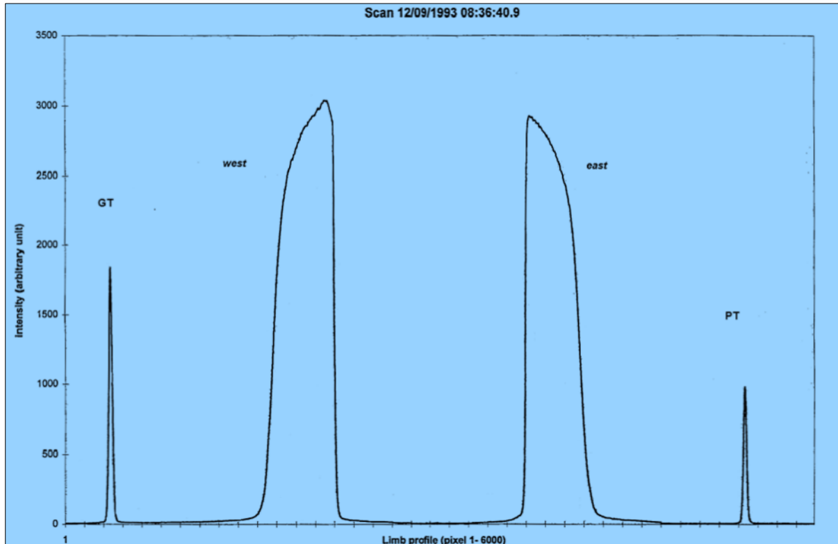
Figure 22: One of the first historical scan, obtained in 1993, showing both solar limbs acquired by the heliometer. The central occulted part was constant and accurately measured to be 1665.1" (courtesy: OCA).
