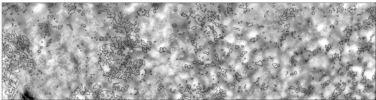
Figure 17: High resolution magnetic fields (black/white isocontours for North/South polarities) in the solar granulation obtained with the MSDP in polarimetric mode (Na D1 5896 Å line) (after Malherbe et al., 2004: 752 ).
