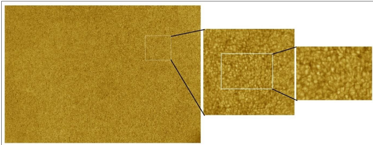
Figure 9: The wide wide field ( 10' \times 10' ) of the CALAS camera for photospheric observations (after Rondi, 2006: 102).
