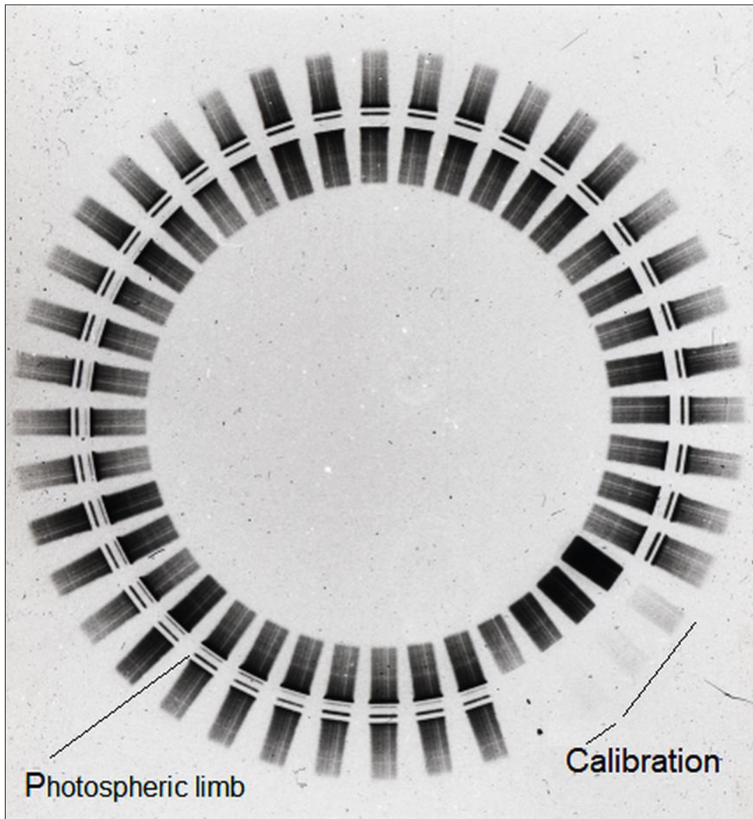
Figure 20: The spectro-coronagraph provided simultaneously the spectra of opposite limbs and was able to explore the corona around the Sun. Plages of calibration were made with successive exposures (courtesy: OCA).
