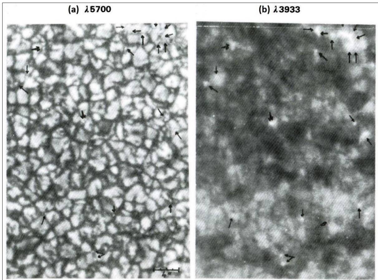
Figure 6: Typical images of the solar granulation obtained at the Pic du Midi Turret-Dome with broad-band filters at 5700 Å, 60 Å FWHM (a), and Cal K 3934 Å, 15 Å FWHM (b). Network bright points are indicated by arrows. The mean size of granules is 1000 km. FOV 30" × 40" (after Muller, 1983: 115).
