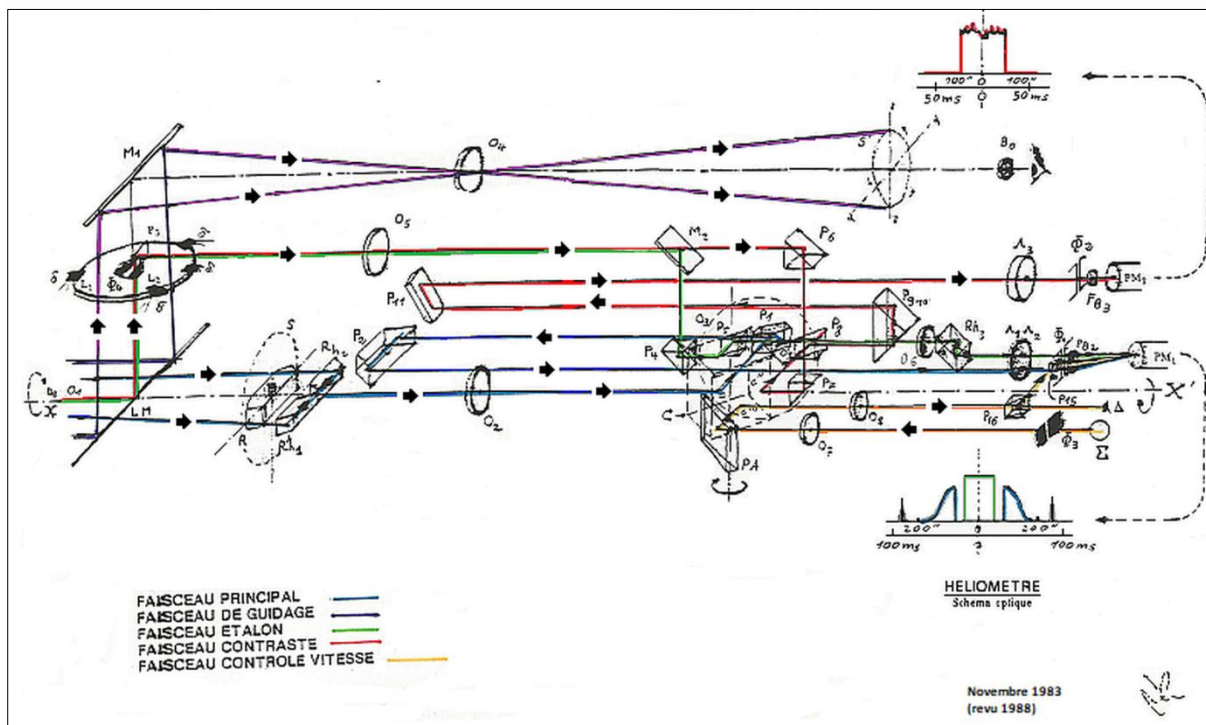
Figure 25: Diagram of the heliometer. Original drawing, dated and signed by J. Rösch, 1983, revised 1988 (courtesy: OCA).
