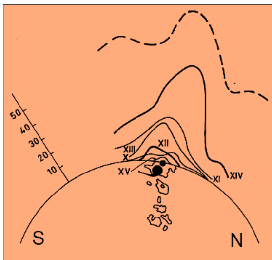
Figure 21: Polar diagram of the emission corona at 60'' from the solar limb, Eastern hemisphere, 19 May 1969, for the six states of ionization of FeX to FeXV. The dashed line represents the intensity of the white corona in arbitrary units. The scale (from 0 to 50) is in millionths of the intensity of a 1 Å band of the solar continuum. The appearance of sunspots has been reproduced from the maps of the Fraunhofer Institute (after Rozelot, 1970: 25).
