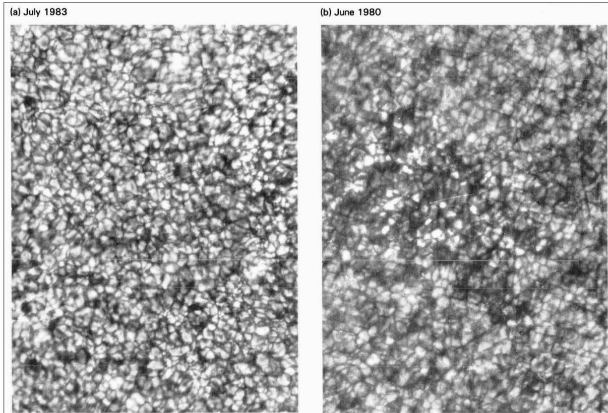
Figure 7: Variation of the photospheric network observed at the Pic du Midi Turret-Dome with a G-band filter (waveband of the CH molecule at 4308 Å, 10 Å FWHM) near solar minimum (a) and solar maximum (b). Bright points (magnetic elements) appear in intergranular lanes. FOV 90" × 120" (after Muller and Roudier, 1984: 36).
