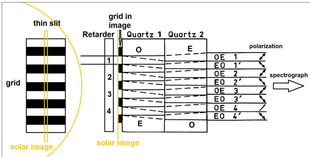
Figure 16: The polarimeter built by M. Semel (1932–2012) is located at the primary focus of the refractor before magnification and injection into the spectrograph. O = ordinary ray; E = extraordinary ray. The grid and the narrow slit are in the solar image at f/13 (after Semel, 1980: 370 ).
