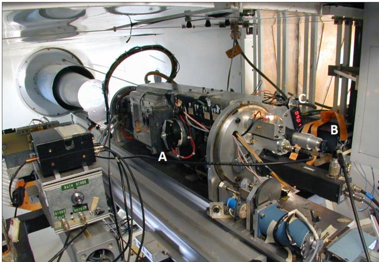
Figure 23: The heliometer mounted in the Turret-Dome. A: servomotor for scanning the light beam (producing the solar limb profiles). B: the output signal recorded through a photomultiplier. C: the digital image slicing counter, a key piece to be sure to pass through the true solar diameter after measuring several chords above and below. The whole system (about 40 kg) was rotating around the optical axis (courtesy: OCA).
