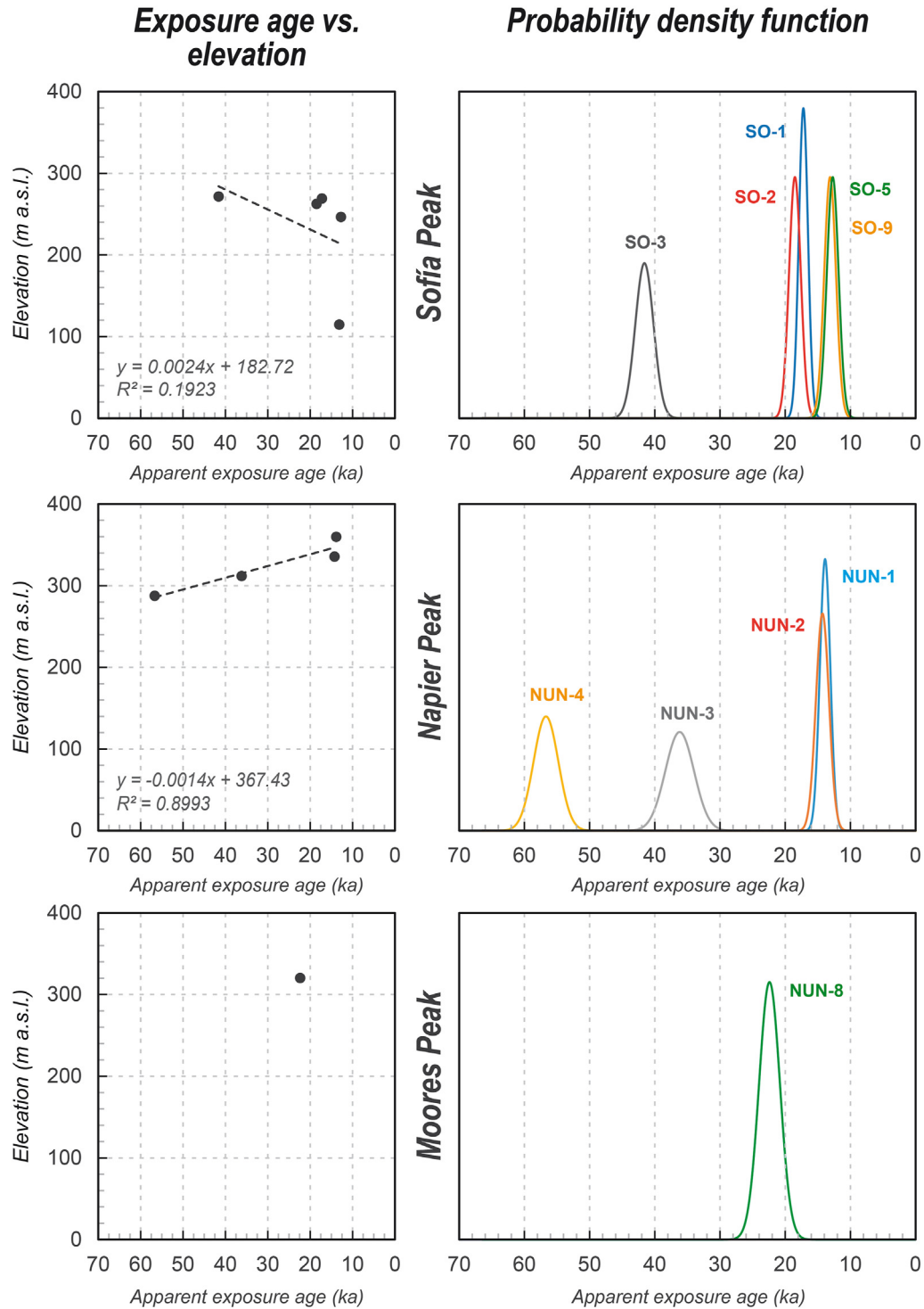
Fig. 5. Probability plots of exposure ages on bedrock at the different sampling sites.
