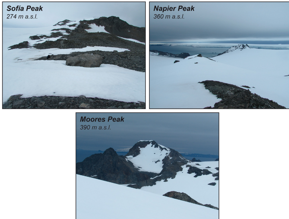
Fig. 3. Pictures of the nunataks studied in this work: Sofia Peak, Napier Peak, and Moores Peak.
