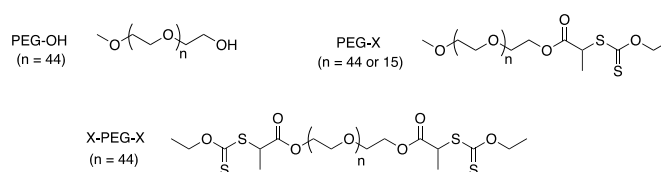
Scheme 1. PEG-based macroCTA used for VDF emulsion polymerization
