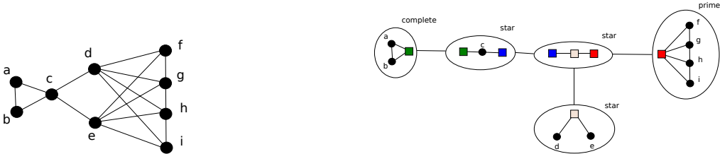
Figure 1: A graph and its split decomposition. Split marker vertices that correspond to a same simple decomposition are identified by two rectangles with the same color.
