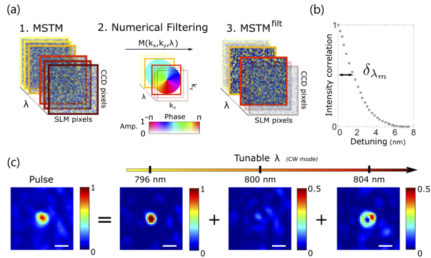
Fig. 2. Principles of spectrally-dependent PSF engineering. (a) Fourier filtering of MSTM with a spectrally-dependent mask M(k_x, k_y, \lambda) gives rise to a new operator, denoted MSTM^{\text{filt}} , which can be used as standard MSTMs. (b) Spectral correlation bandwidth of the scattering medium. The latter is experimentally measured by correlating images acquired while scanning the wavelength of the laser in continuous wave mode by steps of 0.3 nm. Half width at half maximum of this curve ( \delta\lambda_m ) defines the spectral correlation bandwidth of the medium. For this medium we found \delta\lambda_m \approx 1.6 nm. (c) Experimental focusing at two wavelengths with two different and arbitrary chosen PSFs. Scale bars 20 \mu\text{m} .
