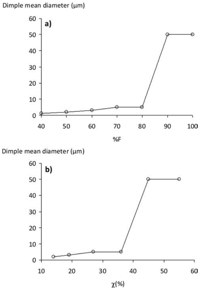
FIGURE 7 Dimple mean diameter versus PVDF contents: (a) wrt \%F ; (b) wrt WFa.
