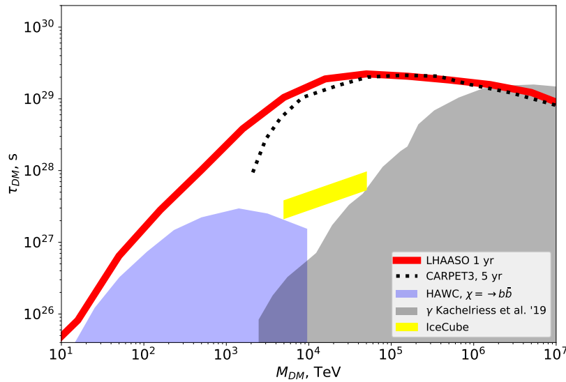
Figure 2: Sensitivity of LHAASO for the measurement of dark matter decay time (for DM decaying into quarks). Yellow band shows the range of decay times for which DM decays give sizable contribution to the IceCube neutrino signal [39]. Blue and gray shaded regions show the existing bounds imposed by HAWC [35] and ultra-high-energy cosmic ray experiments [40]. and dashed curves are from the HAWC search of the DM decay signal in the Fermi Bubble regions [35]. From [31].
