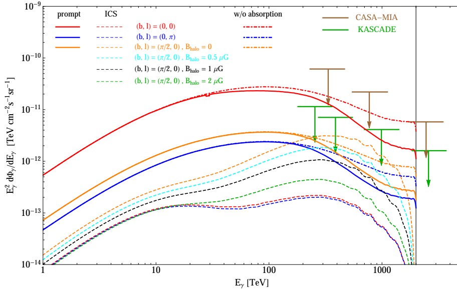
Figure 1: The \gamma -ray flux from DM decay from various directions, with m_{\text{DM}} = 4 PeV and \tau_{\text{DM}} = 10^{28} s, and branching ratios reported in the text. The solid curves show the prompt flux, including the absorption of \gamma -rays, while in the dot-dashed curves the absorption is neglected; different colors represent different directions in the sky. The dashed curves show the IC flux, for various assumptions for the constant halo magnetic field, B_{\text{halo}} , possibly pervading the thick diffusive halo of the Galaxy up to large distances. The green and brown bar lines show the upper bound on \gamma -ray flux from CASA-MIA [37] and KASCADE [38], respectively.
