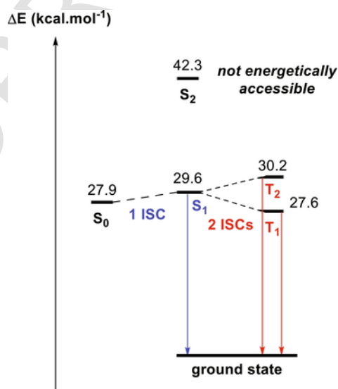
Scheme 6 Schematic energetic diagram for the decomposition of 1,2-dioxetanone. Energies at (T_2)_{\text{min}} ( T_2 computed geometry from the structure of the transition state) relative to the energy of the TS are in kcal mol -1 . Data from Francés-Monerris, A.; Fernández-Galván, I.; Lindh, R.; Roca-Sanjuán, D. Theor. Chem. Acc. 2017 , 136 , article 70.
