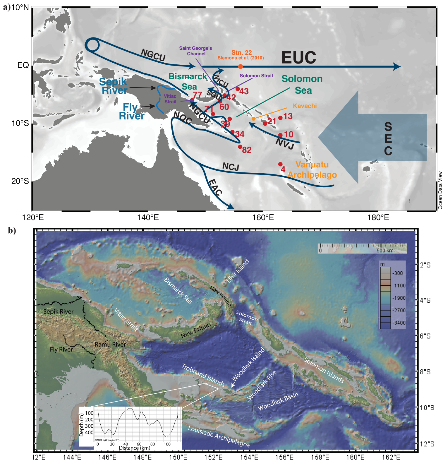
Fig. 1. a) Currents [dark blue; after Germineaud et al. (2016)], rivers (blue text), straits (purple text), and potential point sources (yellow text) to the Solomon Sea. These currents are: Equatorial Undercurrent (EUC); South Equatorial Current (SEC); New Guinea Coastal Undercurrent (NGCU); New Ireland Coastal Undercurrent (NICU); Saint George's Undercurrent (SGU); North Queensland Current (NQC); New Caledonia Jet (NCJ); North Vanuatu Jet (NVJ); East Australian Current (EAC). Red dots and numbers represent stations sampled for Al and Mn. b) Bathymetry of the Woodlark Basin and Trobriand Islands
