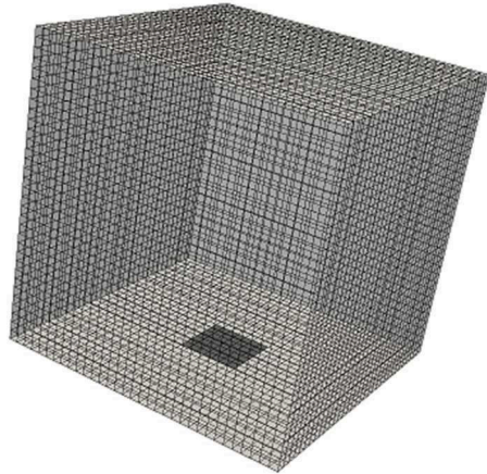
Fig. 13. 3D geometry of the test case corresponding to a cube. The plate burner is the black square (variable size depending on the configuration).
