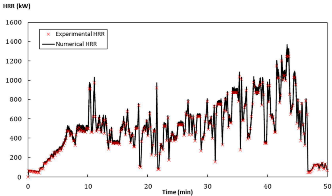
Fig. 15. Comparison between the numerical and the experimental HRR (Heat Release Rates).
