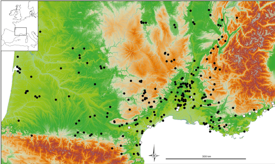
Figure 3: Map of Southern France and distribution of the Early Neolithic sites. In white the Impressa sites. BDA Database ( https://bda.huma-num.fr/ ).
