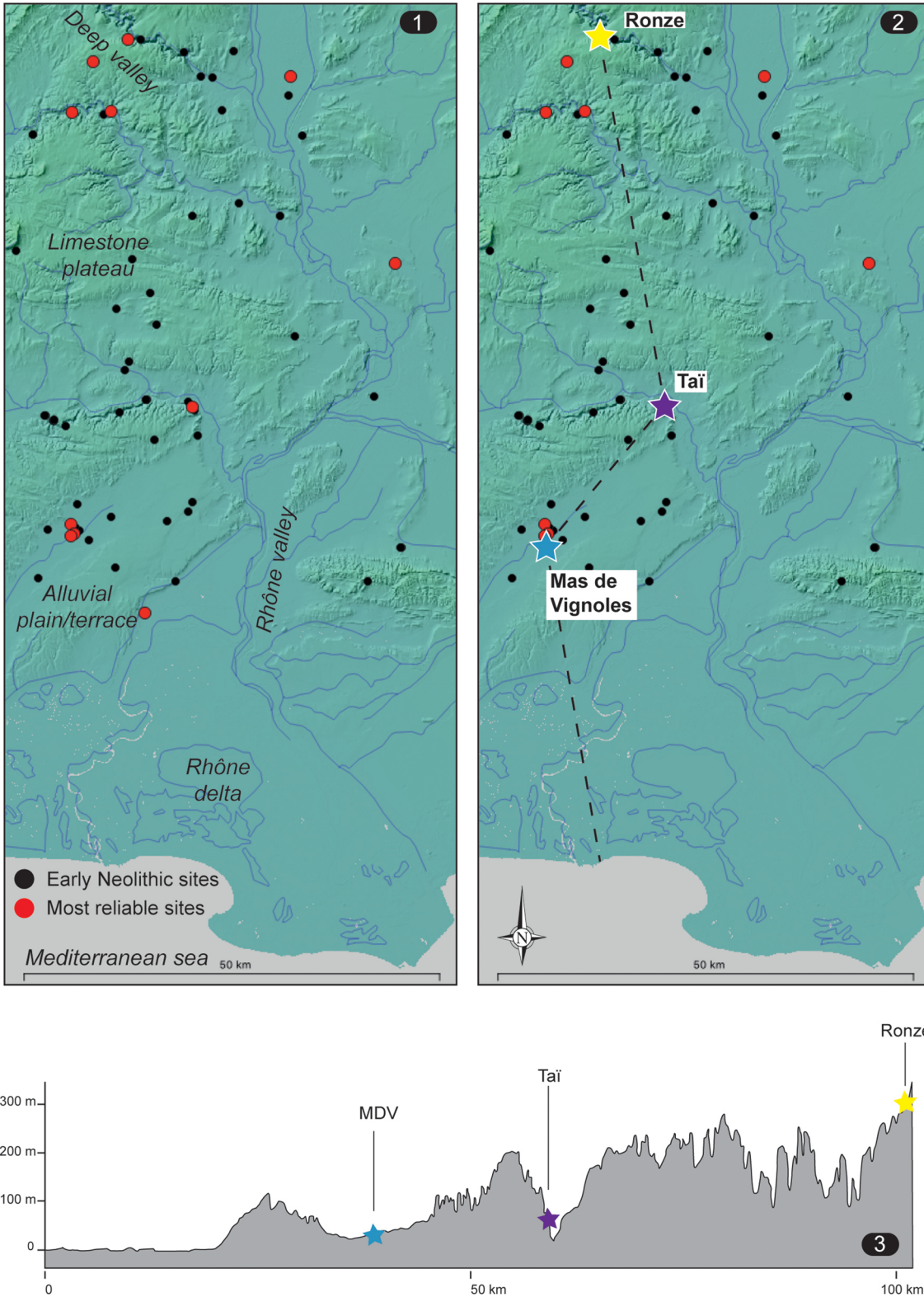
Figure 4: (1) Map illustrating the geographical parameters of the lower Rhône valley, and the location of the Early Neolithic sites (5500–4500 cal. BCE). In red, the most reliable sites (new excavations, multi-proxy data, new radiocarbon dating...). (2) Map illustrating the location of the three sites highlighted in the paper. (3) Schematic topographic location of the three sites highlighted in the paper.
