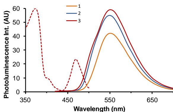
Fig. 7 Excitation spectrum of 3 ( \lambda_{em} = 550 nm, red dotted line) and emission spectra (full lines) of the three complexes 1 (orange line), 2 (blue line) and 3 (red line) as microcrystalline pristine powders. For emission, \lambda_{ex} = 382 nm and intensity proportional to the PLQY.
