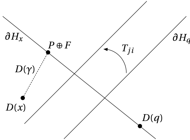
Figure 3: The invisible subspace I .
