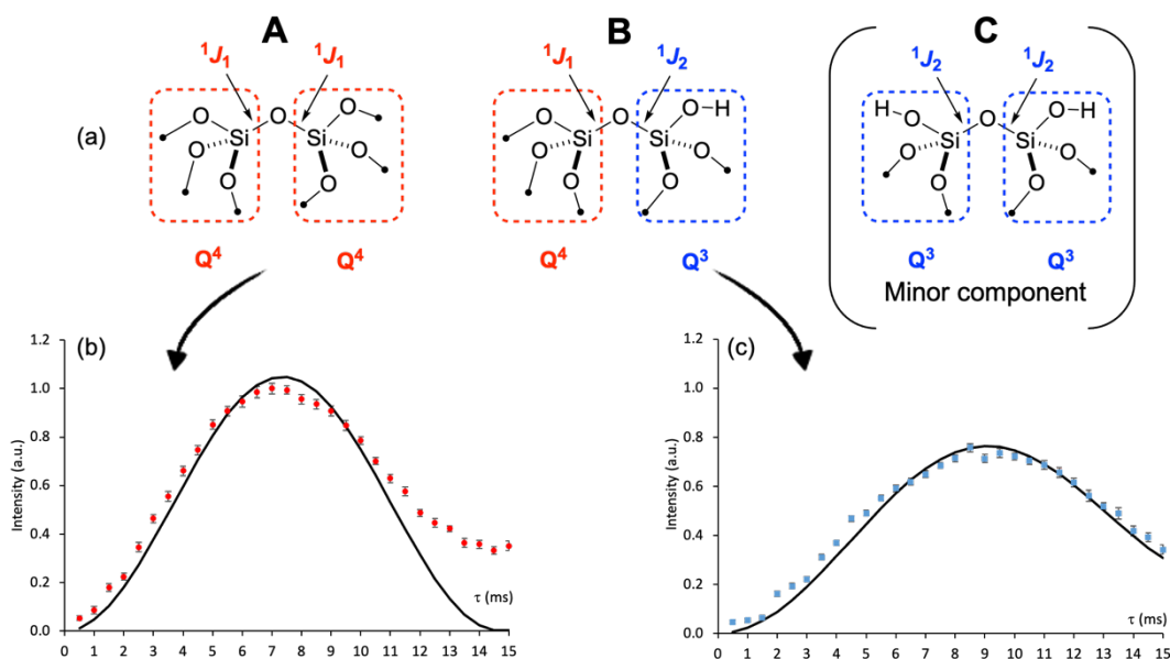
Figure 5 (a) Structure of local siloxane environments. (b,c) Build-up curves of {}^{17}\text{O}\{{}^{29}\text{Si}\} DFS- J -HMQC-QCPMG signals at (b) 34 and (c) 22 ppm assigned to siloxane sites. The red points and the blue squares correspond to the experimental data, whereas the black lines are the simulated curves. The build-up curves were obtained by averaging 10624 transients for each of 30 t_1 increments with a recycle delay \tau_{\text{RD}} = 0.5 s, leading to an experimental time of 45 h. The red and the blue points correspond to the experimental data, whereas the black lines are the simulated curves. The errors bars in the experimental curves subsume the contributions of the noise standard deviation and the error due to the nonlinear fit with DMFIT 46 .
