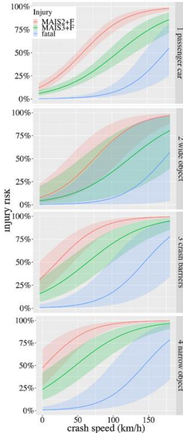
Figure 7: Injury risk curves for different crash opponents
