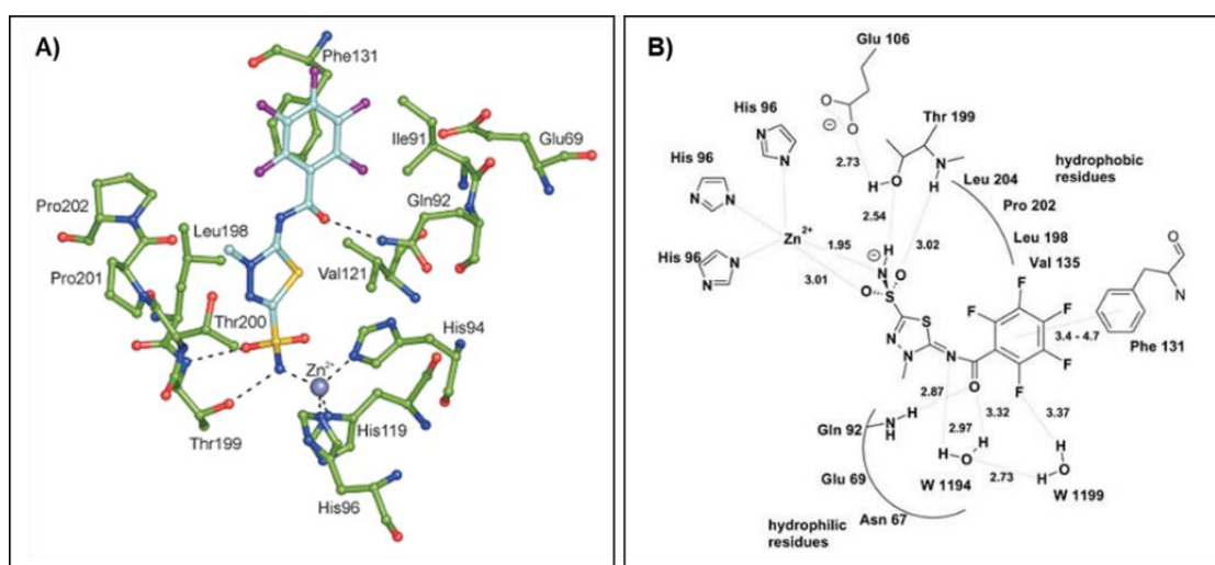
Figure 15. A) CA II/ 67 complex showing the zinc ion coordination, hydrogen bonds and residues participating in the van der Waals interactions with the inhibitor scaffold (distance <math><4.5 \text{ \AA}</math>). B) Schematic representation of PFMZ 67 binding to the CA II active site (numbers represent distances in \text{\AA} ). [21,80]
