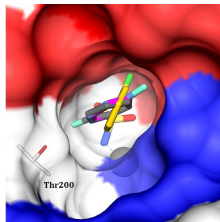
Figure 6. Superposition of CA II/inhibitor adducts: 15 (magenta, PDB 2WEJ), 18 (yellow, PDB 2WEH), 19 (gray, PDB 2WEG) and 20 (blue, PDB 2WEO). Residues delimiting the hydrophobic half are in red, the hydrophilic ones are in blue. Calorimetric data of 15 , 18-20 ( [a]=\text{kcal mol}^{-1} ) [47] and kinITC data of 15 and fluorinated compounds 19 and 20 bound to CA II. [48]
