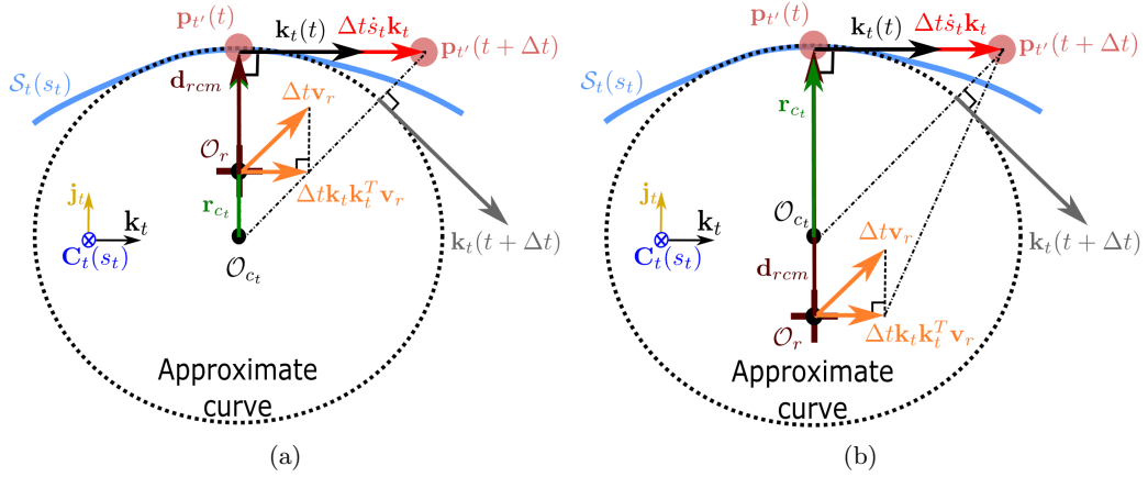
Fig. 9: Zoom on the geometric description of the tool curvature as well as the incision point O_r at the instantaneous positions where (a) the point O_r is located between the two points p_{t'} and O_{c_t} , and (b) the point O_{c_t} is located within the segment formed between O_r and p_{t'} .
